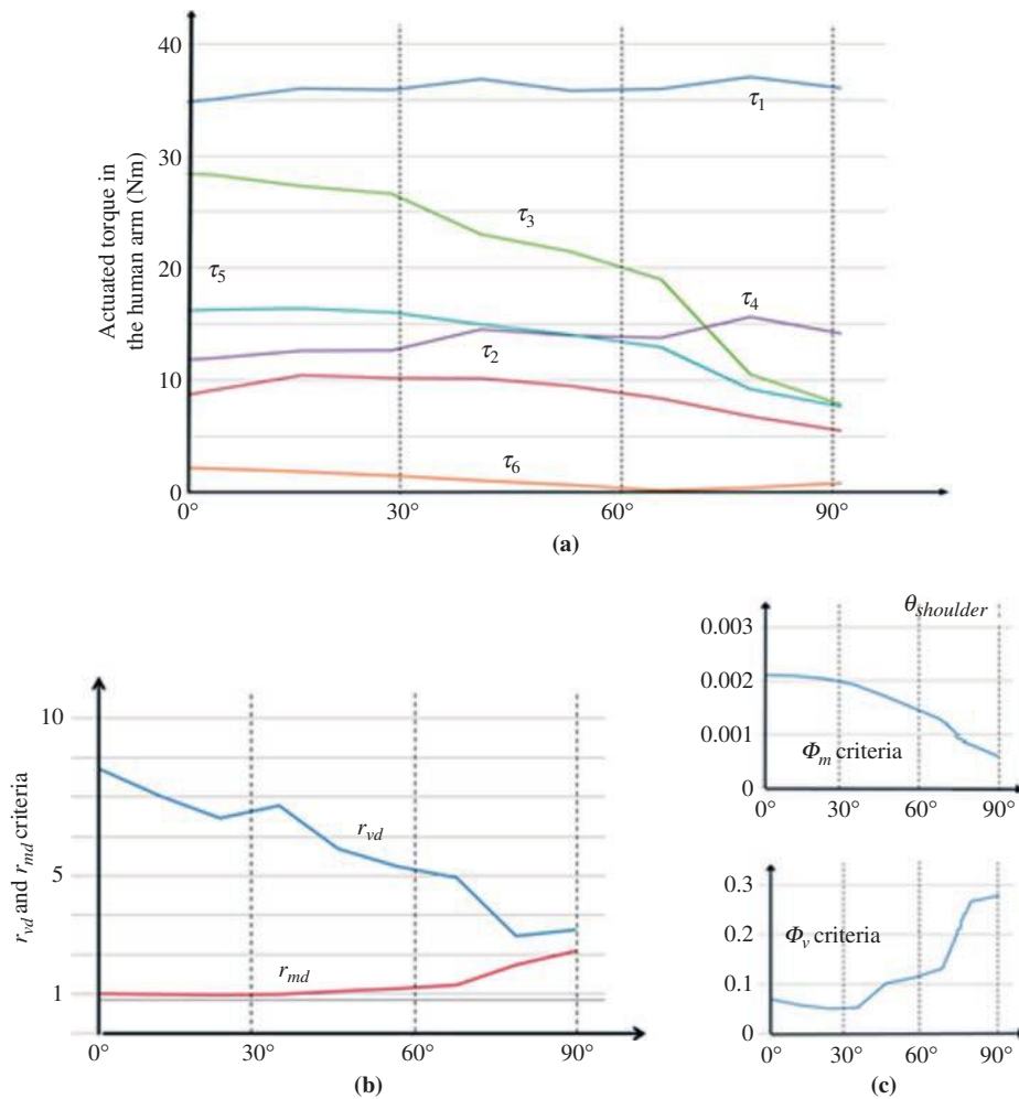
Figure 13 Articular torque and evaluation of \Phi_V and \Phi_m for a force of 50 N and a speed of 50 mm/s
