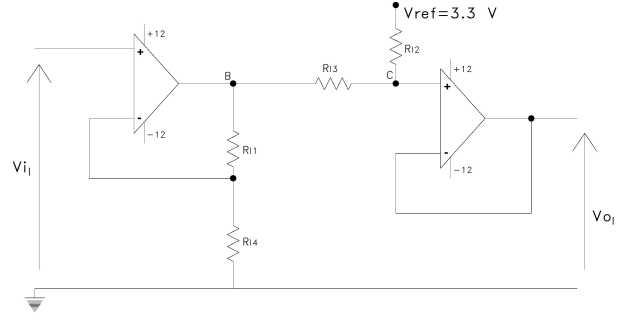
Fig. 3. Current conditioning circuit
