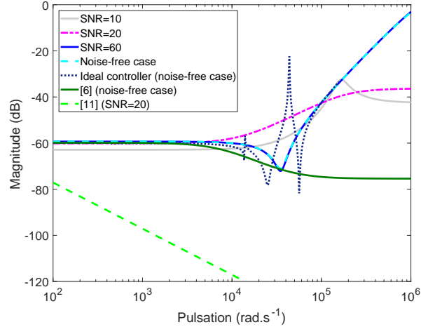
Fig. 2. Frequency response of the “ideal” controller K in the noise-free case (blue dots) and of the identified 2^{nd} -order controllers for different noise levels: SNR=10 (solid grey), SNR=20 (dash-dotted magenta), SNR=60 (solid blue) and in the noise-free case (dashed cyan). The controller obtained in [6] in the noise-free case is indicated by the solid dark green line. The former version of the L-DDC algorithm [11] for SNR=20 gives the controller in dashed light green.
