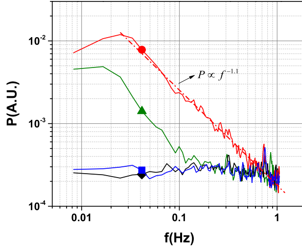
Figure 16: Spectra of the fluctuations of the reduced temperature \theta_r measured by the thermocouple T_4 (see Fig. 1) at various Weissenberg numbers: rhombs (♦) - Wi = 0 , squares (■) - Wi = 0.8 , triangles (▲) - Wi = 7.7 , circle (●) - Wi = 15.4 . The dash - dot line is a guide for the eye, P \propto f^{-1.1} .
