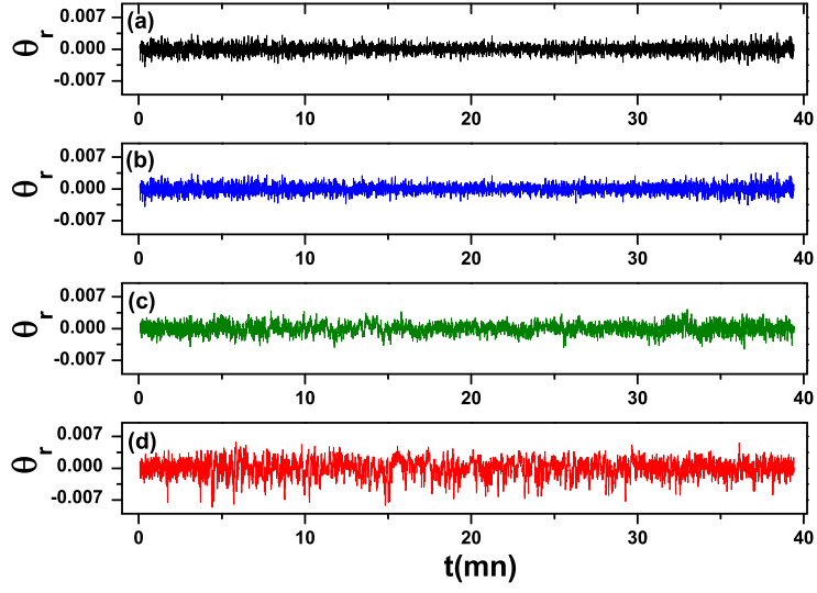
Figure 11: Time series of the fluctuating part of the reduced temperature \theta_r obtained from the measurements of the thermocouple T_4 (see Fig. 1) at various Weissenberg numbers: (a) Wi = 0 (b) Wi = 0.8 , (c) Wi = 7.7 , (d) Wi = 15.4 .
