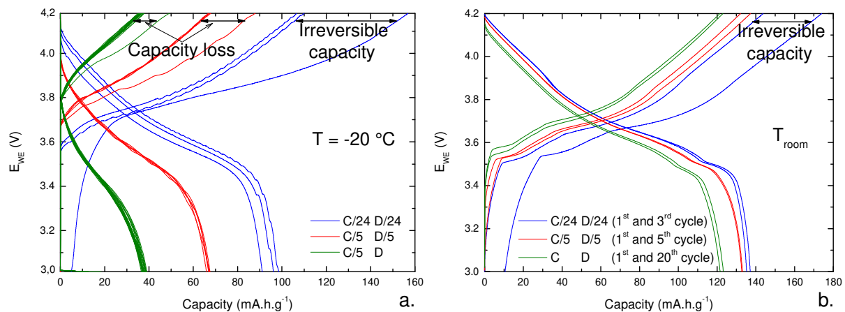
Figure 14. Charge/discharge plots obtained at (a) -20\text{ }^{\circ}\text{C} , and at (b) room temperature ( T_{\text{room}} ). LiTDI-EGM+2%FEC was the electrolyte.
