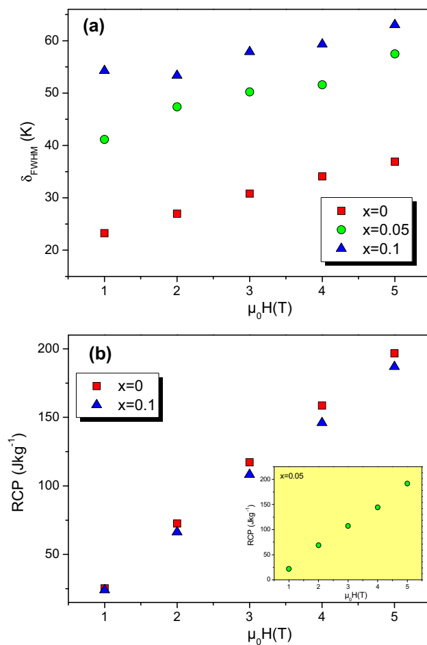
Figure 6. Evolution of (a) \delta_{\text{FWHM}} and (b) RCP vs. magnetic field relative to the \text{Pr}_{0.8-x}\text{Bi}_x\text{Sr}_{0.2}\text{MnO}_3 ( x = 0, 0.05 and 0.1 ) compounds.
