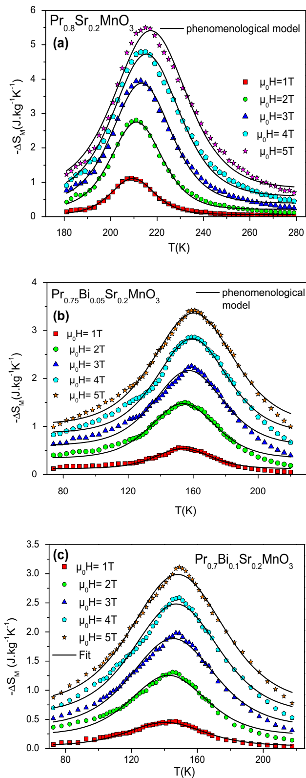
Figure 4. Temperature dependence of the magnetic entropy change |\Delta S_M(T)| under different magnetic applied fields for \text{Pr}_{0.8-x}\text{Bi}_x\text{Sr}_{0.2}\text{MnO}_3 compounds (a) x = 0 , (b) x = 0.05 and (c) x = 0.1 . Solid lines show the predicted values of |\Delta S_M(T)| using table 1 and symbols represent the experimental data.
