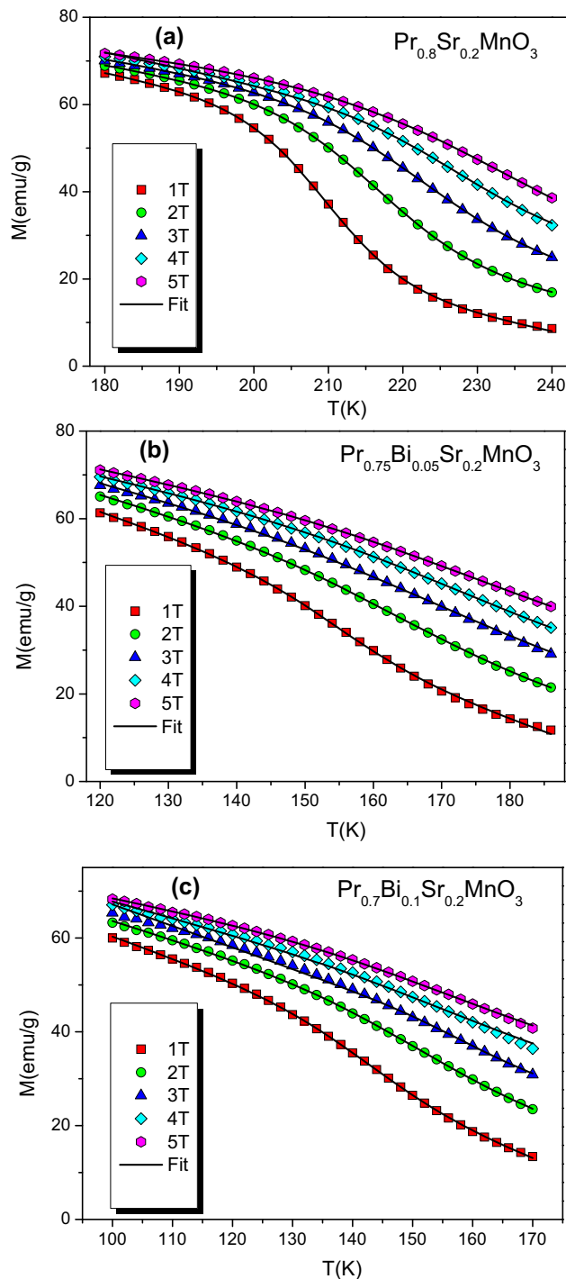
Figure 3. Temperature dependence of the magnetization at different magnetic applied fields for \text{Pr}_{0.8-x}\text{Bi}_x\text{Sr}_{0.2}\text{MnO}_3 compounds ( x = 0, 0.05 and 0.1 ). Symbols represent the experimental data and solid lines represent the simulated results.
