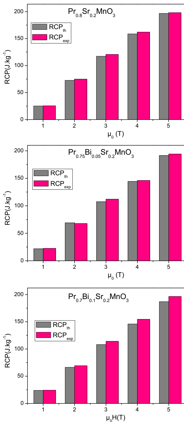
Figure 7. Comparison between RCP values obtained from the phenomenological model ( RCP_{th} ) and those obtained from experimental data ( RCP_{exp} ) for Pr_{0.8-x}Bi_xSr_{0.2}MnO_3 ( x = 0, 0.05 and 0.1 ) compounds.
