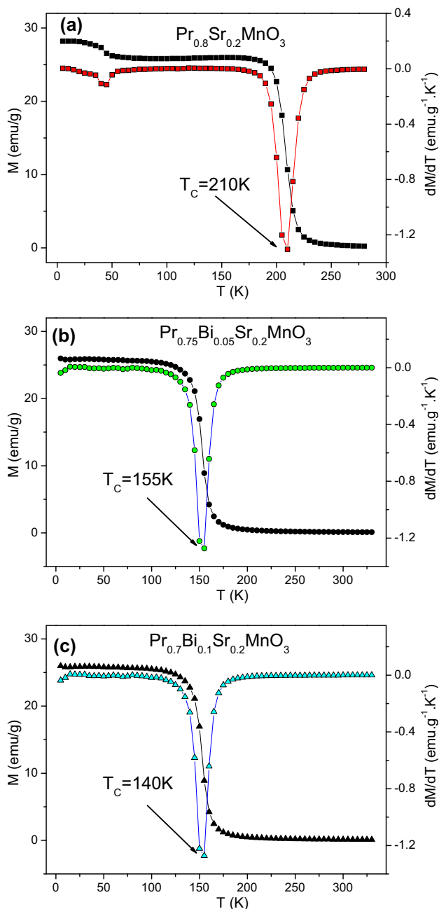
Figure 2. Temperature evolution of the magnetization M(T) determined for the \text{Pr}_{0.8-x}\text{Bi}_x\text{Sr}_{0.2}\text{MnO}_3 compounds under a magnetic applied field of 0.05 T: (a) x = 0 , (b) x = 0.05 and (c) x = 0.1 . The inset of each figure shows the evolution of dM/dT with temperature.
