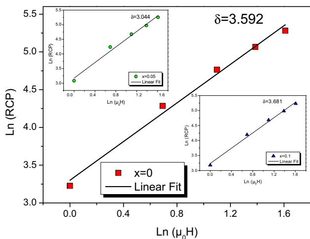
Figure 9. \ln(\text{RCP}) vs. \ln(\mu_0 H) for \text{Pr}_{0.8-x}\text{Bi}_x\text{Sr}_{0.2}\text{MnO}_3 ( x = 0, 0.05 and 0.1 ) compounds.
