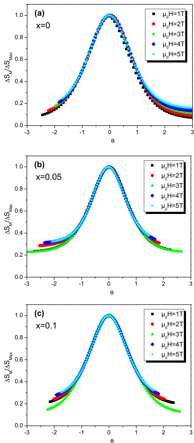
Figure 8. Normalized entropy change vs. rescaled temperature \theta for Pr_{0.8-x}Bi_xSr_{0.2}MnO_3 ( x = 0, 0.05 and 0.1 ) compounds at different applied magnetic fields.
