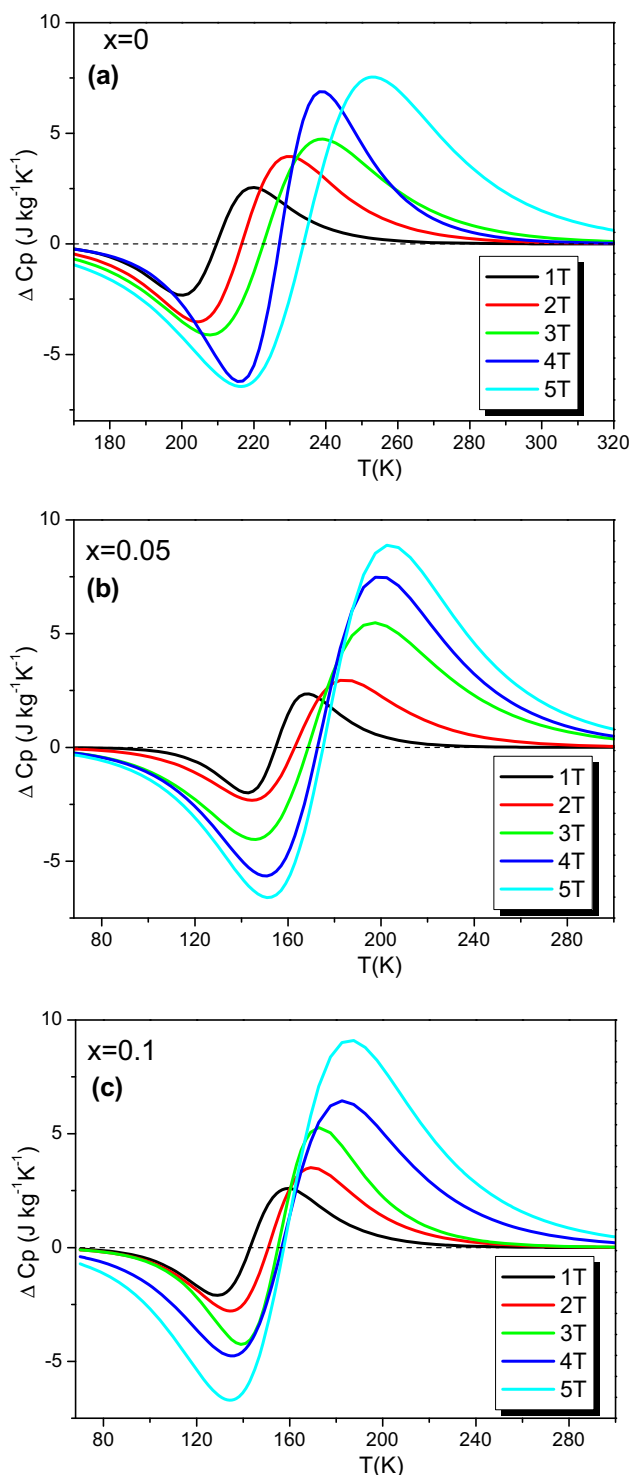
Figure 10. Temperature evolution of the predicted heat capacity under different magnetic applied fields for the \text{Pr}_{0.8-x}\text{Bi}_x\text{Sr}_{0.2}\text{MnO}_3 ( x = 0, 0.05 and 0.1 ) compounds.
