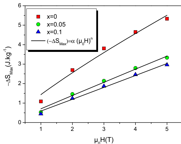
Figure 5. Magnetic field evolution of the maximum entropy change |\Delta S_{\text{Max}}| for \text{Pr}_{0.8-x}\text{Bi}_x\text{Sr}_{0.2}\text{MnO}_3 ( x = 0, 0.05 and 0.1 ) compounds.
