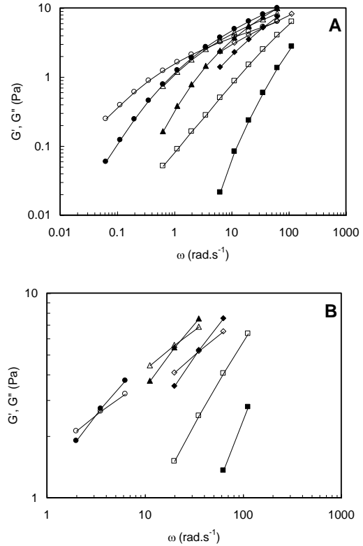
Figure 1. (A) Evolution of the storage (filled symbols) and loss (open symbols) shear moduli within the linear regime for the 1wt% PEO ( M_w = 5 \times 10^6 g.mol -1 ) solution containing various amounts of CNC (on the PEO basis) as a function of the frequency: 0 wt% (●,○), 3 wt% (▲,△), 6 wt% (■,□) and 9 wt% (◆,◇). (B) Zoom on the experimental values surrounding the cross over zone.
