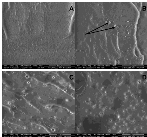
Figure 5. SEMs of (A) neat LDPE, and LDPE reinforced with (B) 9 wt% CNC, (C) 6 wt% PEO-adsorbed CNC ( 3.5 \times 10^4 g.mol -1 ), and (D) 9 wt% PEO-adsorbed CNC ( 5 \times 10^6 g.mol -1 ).
