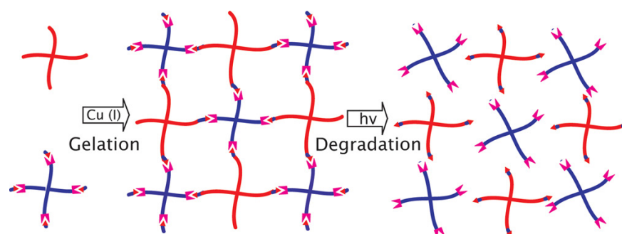
Fig. 14 Example of the destabilization of a chemically crosslinked gel [110] [Reprinted with permission from M.A. Azagarsamy, D.D. McKinnon, D.L. Alge, K.S. Anseth, Coumarin-Based Photodegradable Hydrogel: Design, Synthesis, Gelation, and Degradation Kinetics , ACS Macro Lett. 3 (2014) 515–519 Copyright (2014) American Chemical Society.]
