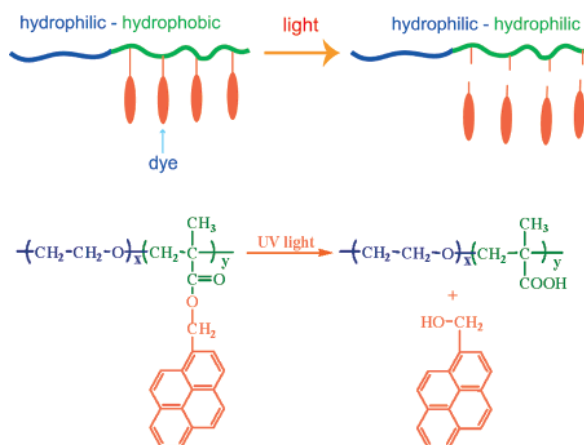
Fig. 9 Release of a hydrophobic group induced particle by destabilization [74] [Reprinted with permission from J. Jiang, X. Tong, Y. Zhao, A New Design for Light-Breakable Polymer Micelles, J. Am. Chem. Soc. 127 (2005) 8290–8291. Copyright (2005) American Chemical Society.]
