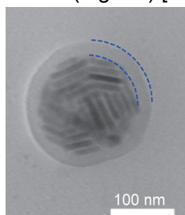
Fig. 16 \text{Cu}_{1.75}\text{S} nanocrystals encapsulated in a temperature-responsive polymer [13] [ Reprinted by permission from Springer Nature: Nanoresearch, S. Huang, J. Liu, Q. He, H. Chen, J. Cui, S. Xu, Y. Zhao, C. Chen, L. Wang, Smart \text{Cu}_{1.75} nanocapsules with high and stable photothermal efficiency for NIR photo-triggered drug release, Nano Res. 8 (2015) 4038–4047 copyrights (2015)]
