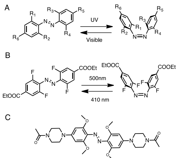
Fig. 7 A) Reversible azobenzene trans-cis isomerization under UV and visible light B) o -Fluoro-azobenzene showing a red shift in absorption and a stable cis isomer ( \tau_{1/2} =2 years) [82] C) Azobenzene derivative showing particularly large red shifting [83].
