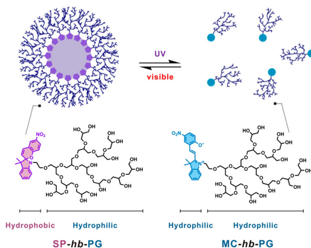
Fig. 10 Spiropyran hydrophilicity switch inducing particles destabilization [96] [Reprinted with permission from S. Son, E. Shin, B.-S. Kim, Light-Responsive Micelles of Spiropyran Initiated Hyperbranched Polyglycerol for Smart Drug Delivery , Biomacromolecules . 15 (2014) 628–634. Copyright (2014) American Chemical Society.]
