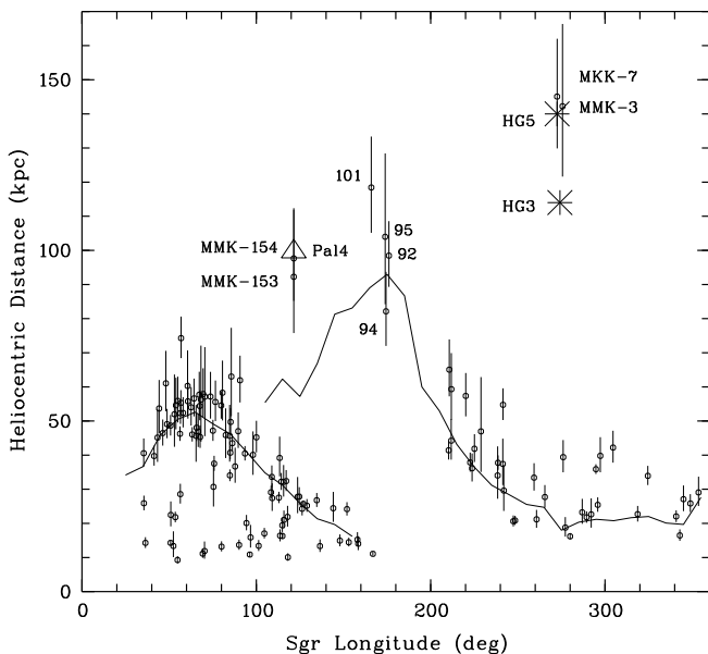
Fig. 9. Heliocentric distance as a function of the Sgr longitude. Only stars within 13 degrees from the Sgr orbit plane are plotted. The continuous line is the average position of the Sgr arms given by Hernitschek et al. (2017). The 1\sigma scatter of this RR Lyrae positions is \sim 5 kpc. The globular cluster Pal 4 is indicated by a triangle. Two carbon stars, HG5 and HG3, are plotted with asterisks.
