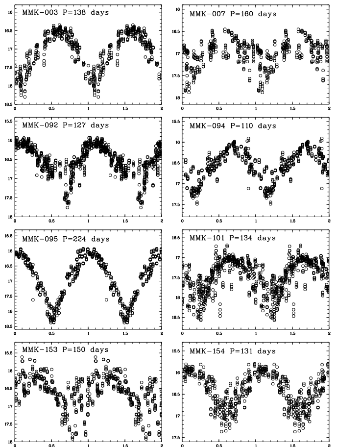
Fig. 10. Plots of Catalina magnitude as a function of phase, for labelled stars in Fig. 9. The lightcurves at bottom refer to two members of the Pal 4 globular cluster.
