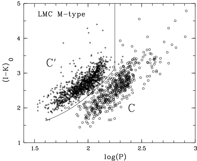
Fig. 5. Plot of the (I - K_s)_0 colour index versus period (in days) for oxygen-rich MSRA variables of the LMC. The curved line separating sequence C and C' is y = ax^2 + b where x = \log(P) - 1.2 , a = 2.3 , b = 1.45 . The vertical line corresponds to P = 178 days.
