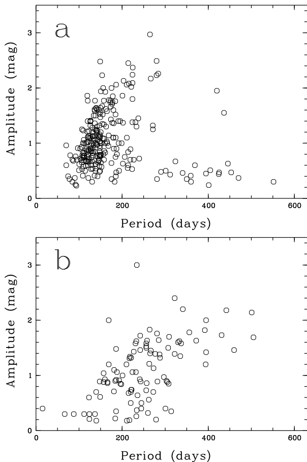
Fig. 3. Catalina amplitudes plotted as a function of pulsation periods for MSRA in the halo. All stars plotted here have |Z| > 5 kpc. We show in panel a our sample stars obeying (J - K_s)_0 < 1.3 . In panel b , we show carbon stars. Note the large difference of these two distributions, strongly suggesting that most of the stars in the upper panel are not carbon rich. All stars plotted here have |Z| > 5 kpc.
