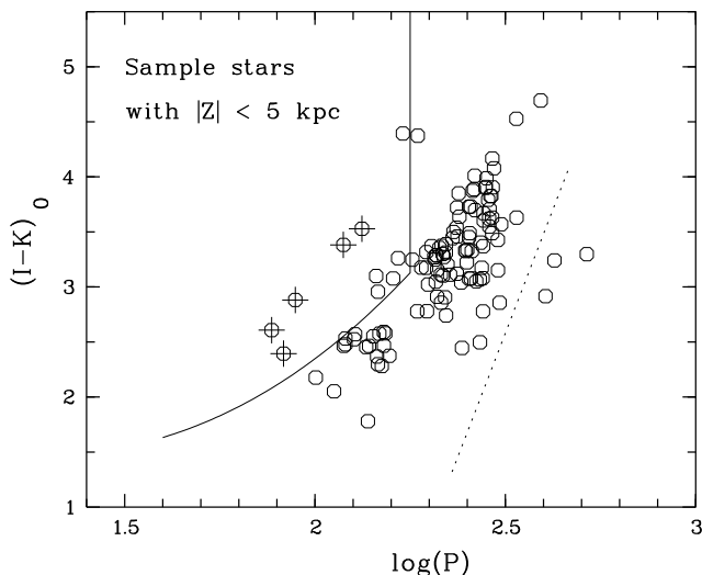
Fig. 7. Same as Fig. 6 for stars of our sample being closer than 5 kpc from the galactic plane.
