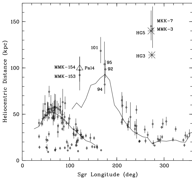
Fig. 9. Heliocentric distance as a function of the Sgr longitude. Only stars within 13 degrees from the Sgr orbit plane are plotted. The continuous line is the average position of the RR Lyr variables of the Sgr arms given by Hernitschek et al. (2017). The 1\sigma scatter of this RR Lyrae positions is \sim 5 kpc. The globular cluster Pal 4 is indicated by a triangle. Two carbon stars, HG5 and HG3, are plotted with asterisks.
