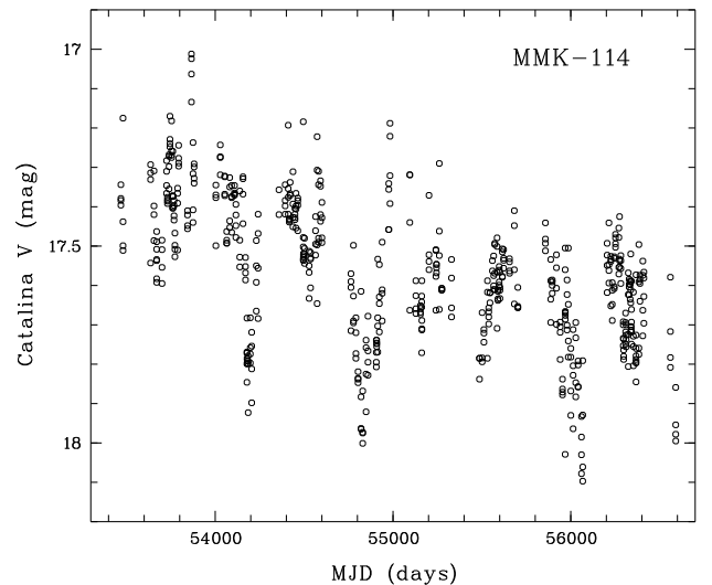
Fig. 12. Light curve of MMK-114 (see text).
