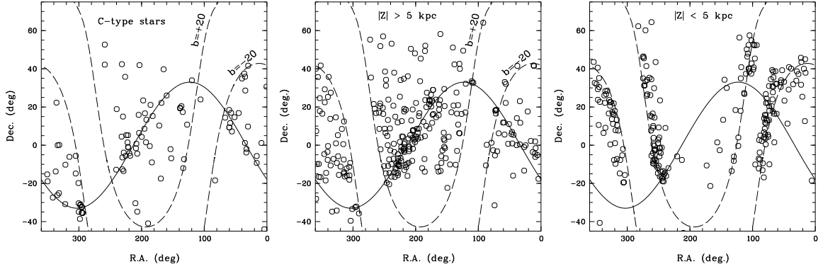
Fig. 4. Apparent positions of pulsating AGB stars in equatorial coordinates. In the left panel, we plot all known C stars that are periodic and have |Z| > 5 kpc. The sinusoid is an eye fit to the majority of these C stars. In the middle panel, we plot stars of our sample (M type) having |Z| > 5 kpc. In the right panel, we plot stars of our sample having |Z| < 5 kpc. Dashed lines indicate |b| = 20^\circ . Note that M stars are more numerous than C stars along the Sgr arms.
