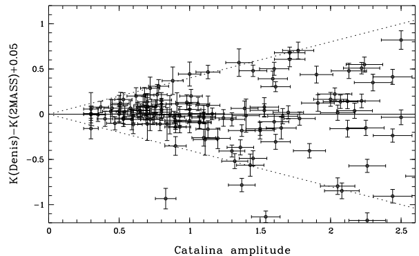
Fig. 8. Difference between K_{\text{DENIS}} and K_{2\text{MASS}} as a function of the Catalina amplitude for 136 stars of our sample obeying K_{2\text{MASS}} > 5 . This diagram suggests the K -band amplitude to be around 0.4 \times the V -band Catalina amplitude, as indicated by dotted lines.
