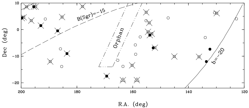
Fig. 11. Close-up on the region of the group of stars seen at R.A. \sim 160^\circ . M stars and C stars are plotted with open and filled circles, respectively. Two triangles at bottom are pair 6 of Stackenbourg (2009). Overplotted crosses are stars more distant than 25 kpc from the Sun. Those at the upper left corner belong to Sgr arm. The Orphan stream position is indicated.
