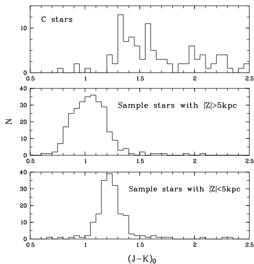
Fig. 1. Histogram of (J - K)_0 of long period variables. Top panel: halo C stars. Middle panel: stars in our sample for which the height |Z| from the galactic plane is larger than 5 kpc. Lower panel: as middle panel, but |Z| < 5 kpc. In none of the panels do we include irregular variables, with no well-defined periodicity (they are ignored in this paper).
