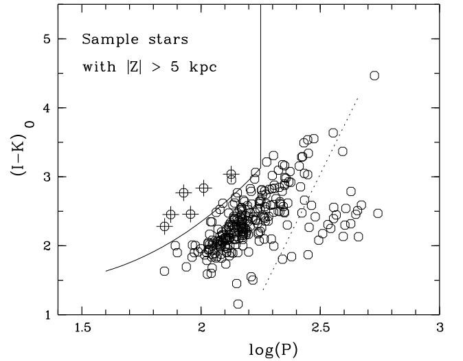
Fig. 6. Plot of (I - K_s)_0 versus period (in days) for our sample stars located at more than 5 kpc from the galactic plane. The curved line is the same as for LMC. Stars with an overplotted cross are attributed to sequence C'. Stars to the right of dotted line are considered to belong to sequence D.
