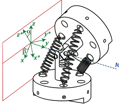
Fig. 6. Representation of tilt ( \alpha ) and azimuth ( \beta ) angles on the universal joint
