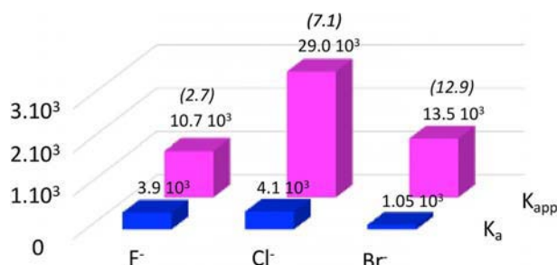
Figure 4. Comparison of binding constants for anions@ 2 ( K_a , blue) and anion@ [\text{2-Me}_4\text{N}^+] ( K_{app} , pink) complexes. Cooperativity factors are given in parentheses.
