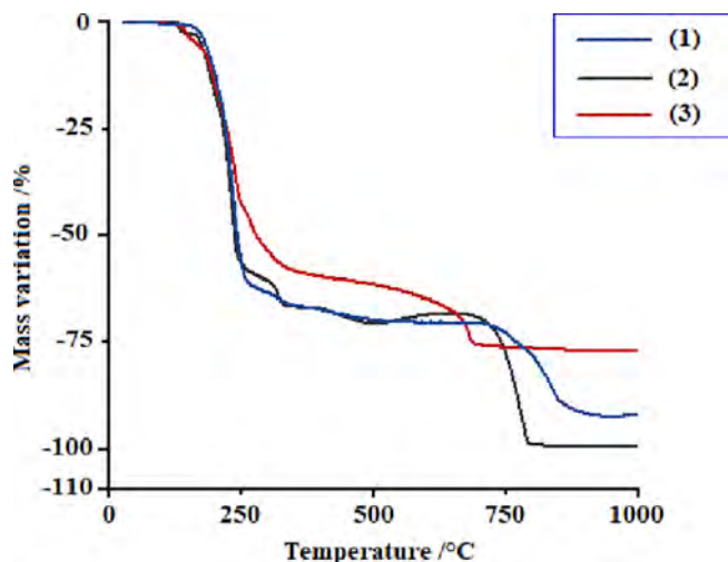
Fig. 3. TGA diagrams of compounds (1), (2) and (3).
