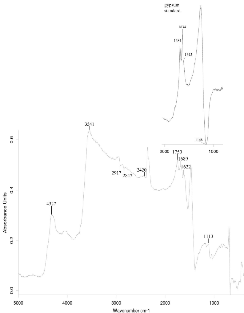
Figure 12 FTIR spectrum in pseudo-absorbance of the ground layer of Ritratto di Giulio Mylius (Villa Vigoni), suggesting the presence of white lead (3541, 2420, 1750 \text{cm}^{-1} ), siccativ oil (4327, 2917, 2847, 1750 \text{cm}^{-1} ) and gypsum (1689, 1622, 1113 \text{cm}^{-1} ). The peculiar peaks of gypsum reference are also shown.
