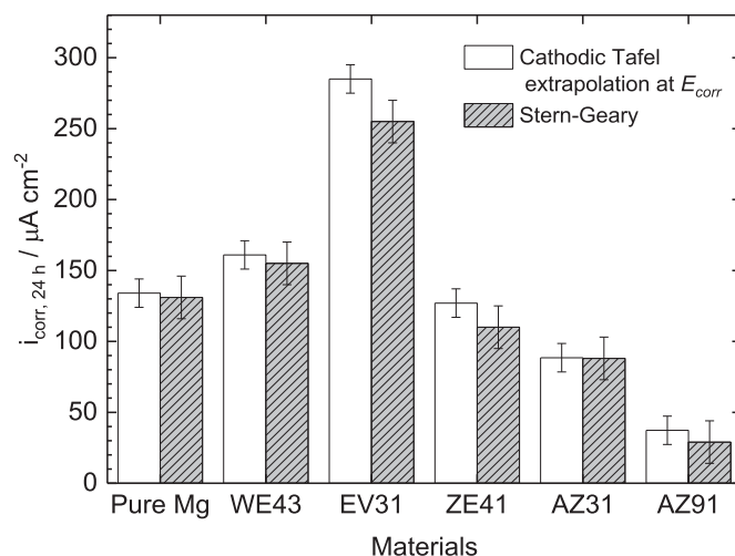
Fig. 9. Comparison of the instantaneous corrosion current densities for the Mg alloys and the pure Mg obtained from the extrapolation of the cathodic Tafel plot at E_{\text{corr}} (Fig. 3) or from the Stern-Geary relationship (Eq. (2)) after 24h of immersion in a 0.1M \text{Na}_2\text{SO}_4 .
