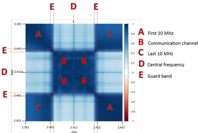
Fig. 6: Frequencies correlation.
