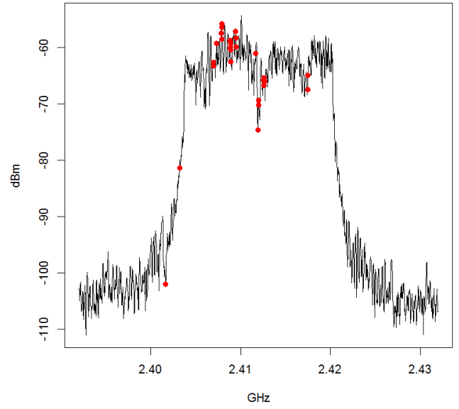
Fig. 9: Best Frequency.
