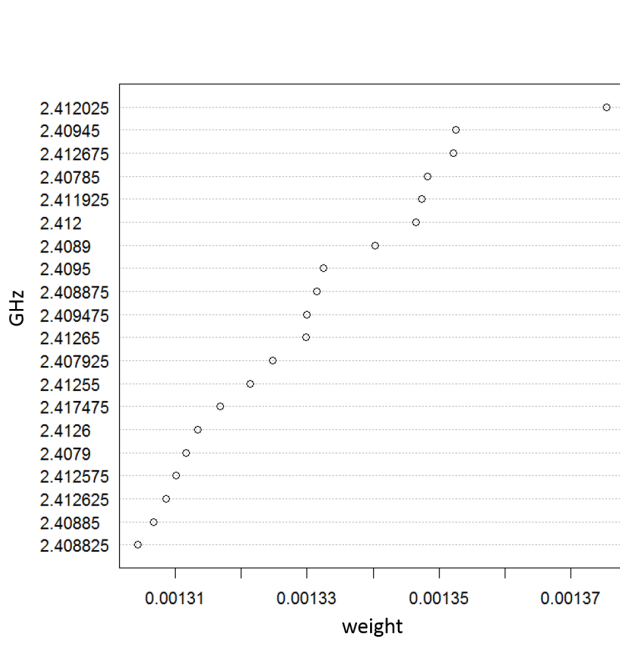
Fig. 8: Weight of the 20 first relevant frequencies.
