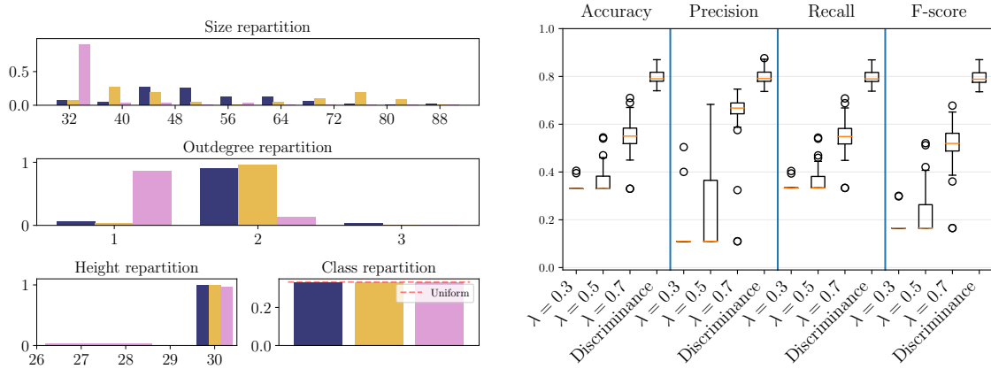
Figure 16: Description of the Faure et al. data set (300 trees, left) and classification results (right).
