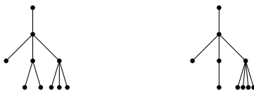
Figure 1: Two trees T_0 and T_1 that fulfill conditions 1 and 2.
