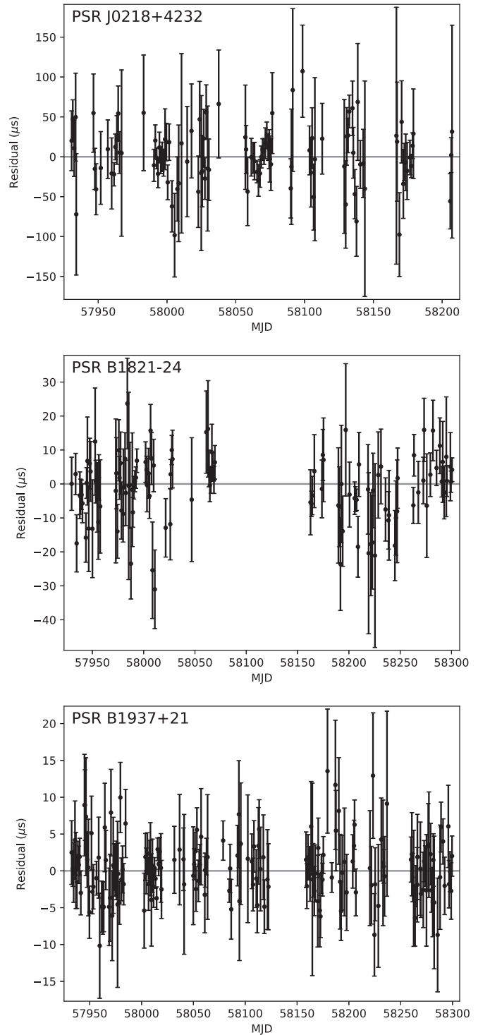
Figure 12. NICER timing residuals with respect to the final timing solutions after refitting the rotational period, period derivative, and in the case of PSR J0218+4232, also binary parameters using only NICER TOAs, as described in Section 6.
