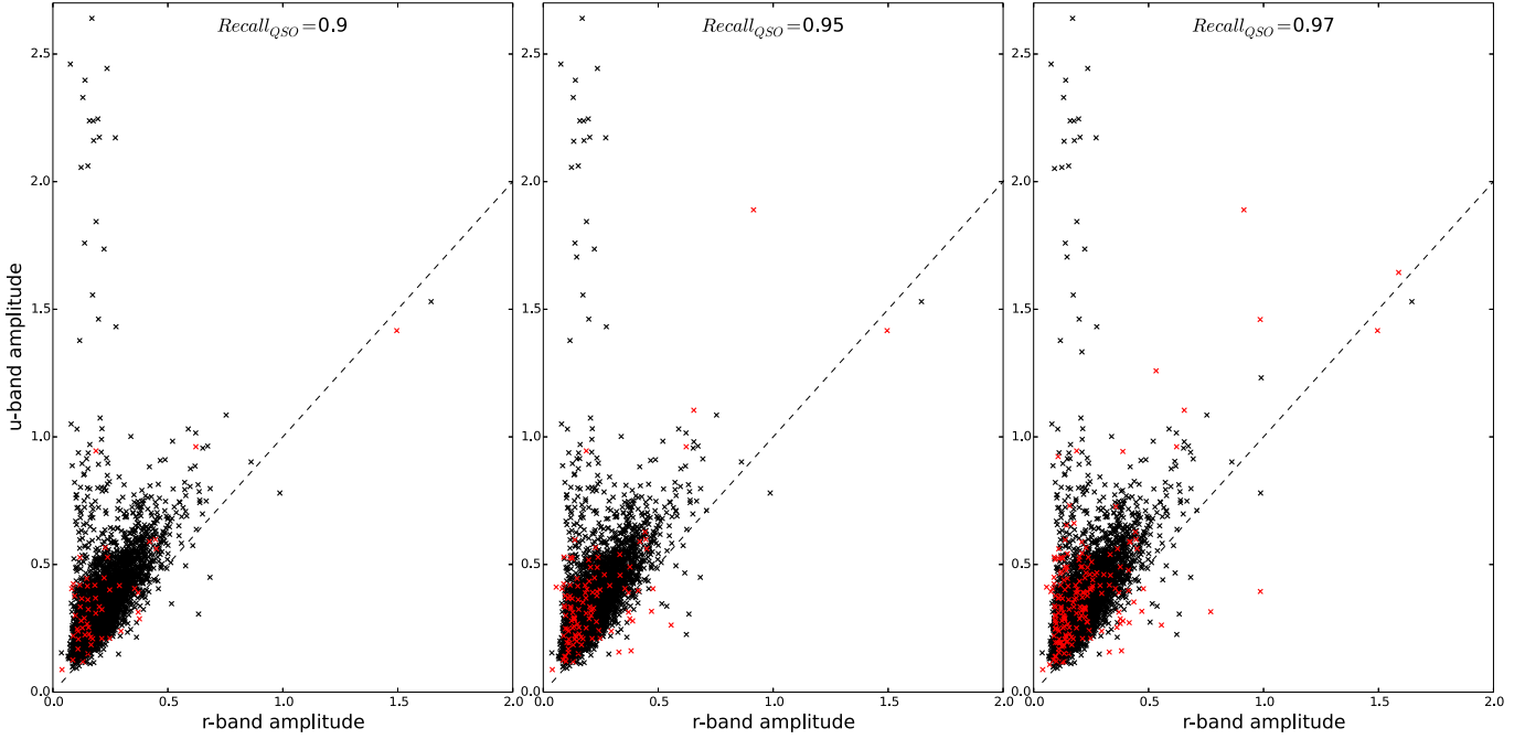
Fig. 8. Amplitudes of variation of quasars detected by the CNN from the u -band filter against those from the r -band filter at three different recalls: 0.90, 0.95, and 0.97. The black crosses represent all the known quasars during the testing phase. The red crosses are the 175 new quasar candidates. The dashed lines represent the line y = x . The quasars show larger variation amplitudes in bluer-bands. This tendency highlights a strong wavelength dependence.
