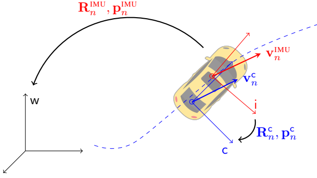
Fig. 2. The coordinate systems that are used in the paper. The IMU pose (\mathbf{R}_n^{\text{IMU}}, \mathbf{p}_n^{\text{IMU}}) maps vectors expressed in the IMU frame i (red) to the world frame w (black). The IMU frame is attached to the vehicle and misaligned with the car frame c (blue). The pose between the car and inertial frames (\mathbf{R}_n^c, \mathbf{p}_n^c) is unknown. IMU velocity \mathbf{v}_n^{\text{IMU}} and car velocity \mathbf{v}_n^c are respectively expressed in the world frame and in the car frame.
