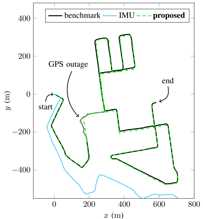
Fig. 1. Trajectory results on seq. 08 (drive #28, 2011/09/30) [3] of the KITTI dataset. The proposed method (green) accurately follows the benchmark trajectory for the entire sequence (4.2 km, 9 min), whereas the pure IMU integration (cyan) quickly diverges. Both methods use only IMU signals and are initialized with the benchmark pose and velocity. We see during the GPS outage that occurs in this sequence, our solution keeps estimating accurately the trajectory.
