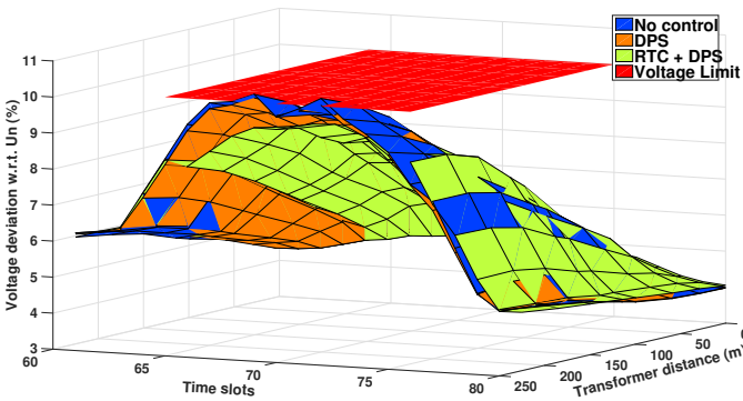
Fig. 1. Maximum voltage deviations along the feeder.
