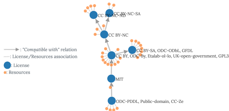
(a) Compatibility graph of the ODRL_CaLi ordering for some licensed RDF datasets.
