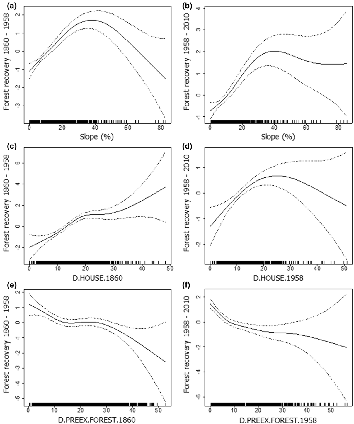
Fig. 5 Univariate smoothed terms of slope, distance from houses and distance from pre-existing forest in relation to forest recovery from 1860 to 1958 ( a , c , e ) and from 1958 to 2010 ( b , d , f ). Estimates are shown by solid lines, confidence intervals are
