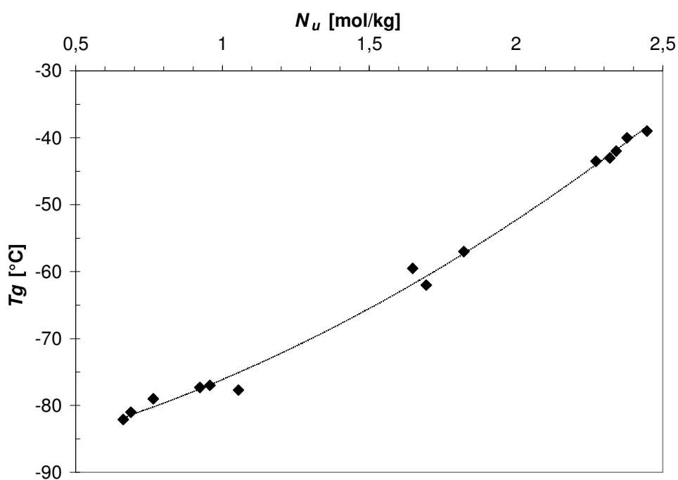
Fig. 10. Dependence of T_g (determined from the second DSC scans) versus the weight concentration of the urethane groups N_u determined for the PU networks described in this work and in ref. 17 (solid line: empirical 2 nd power law T_g = -89.5 + 8.22N_u + 5.20N_u^2 ).
