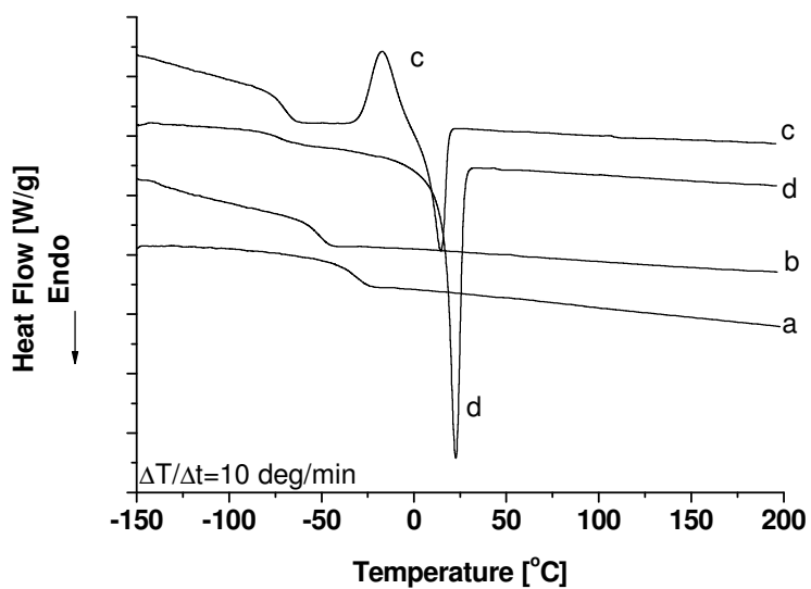
Fig. 3. DSC spectra (second scans) for the PU systems with different lengths of macrodiol: a) 20-T650, b) 20-T1000, c) 20-T2000 and d) 20-T2900.
