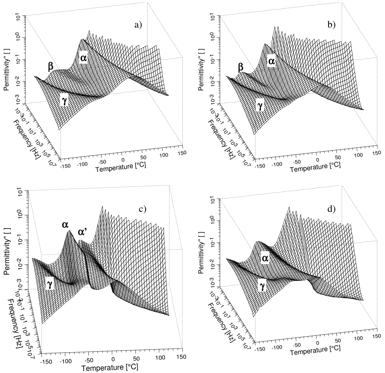
Fig. 4. Frequency and temperature dependencies of the dielectric permittivity imaginary part for the PU networks based on macrodiol with different lengths, but constant n = 20 : a) 20-T650, b) 20-T1000, c) 20-T2000 and d) 20-T2900.
