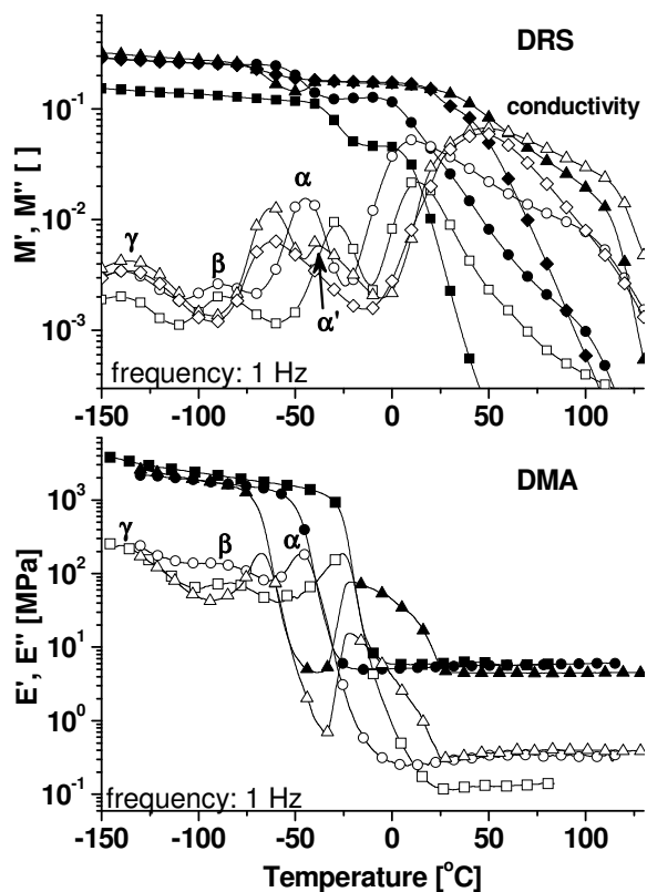
Fig. 5. DRS and DMA spectra for the PU networks based on macrodiols with different molecular weight but constant n = 20 : 20-T650 (■, □), 20-T1000 (●, ○), 20-T2000 (▲, △) and 20-T2900 (◆, ◇). Full points – real part, open points – imaginary part of the moduli.
