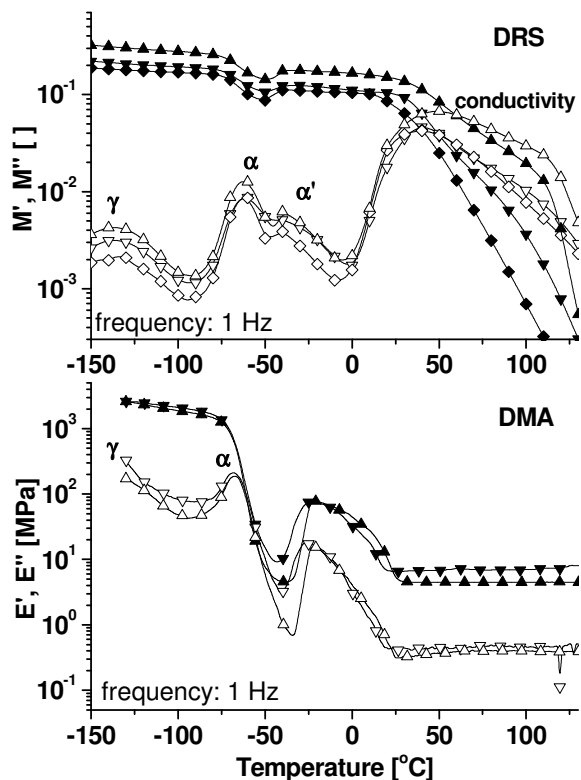
Fig. 7. DRS and DMA spectra for PU networks based on the same macrodiol Terathane ® 2000 but with different numbers of repeating units n : 4-T2000 ( \blacktriangledown, \blacktriangledown ), 10-T2000 ( \blacklozenge, \blacklozenge ) and 20-T2000 ( \blacktriangle, \blacktriangle ). Full points – real part, open points – imaginary part of the moduli.
