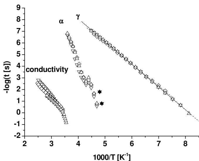
Fig. 8. Activation map for PU networks based on the same macrodiol Terathane ® 2000 but with different numbers of repeating units n : 4-T2000 ( \blacktriangledown, \blacktriangledown ), 10-T2000 ( \blacklozenge, \blacklozenge ) and 20-T2000 ( \blacktriangle, \blacktriangle ). Open points – DRS; full points – DMA.
