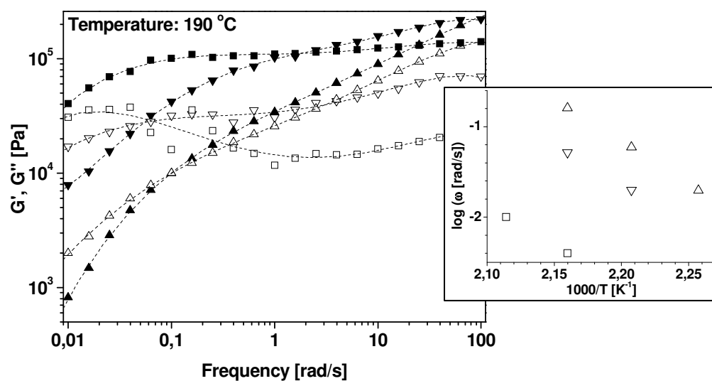
Fig. 9. Rheological measurements for the samples: 4-T650 (■,□), 4-T2000 (▼,▽) and 20-T2000 (▲,△). Full points – real part, open points – imaginary part of the shear modulus G . Inset diagram shows the frequency-temperature dependence of the flowing points.
