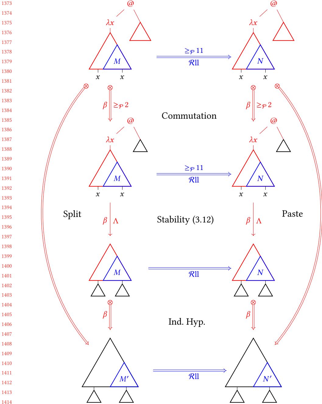
Fig. 6. Construction of a decreasing diagram for peak: Lemma 5.14
