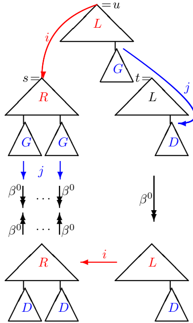
■ Figure 1 Ancestor peaks in rewrite theories. L, G stand for terms rewriting to R, D , using a red rule in \mathcal{R}l and a blue rule in \mathcal{R}l \cup \beta .
