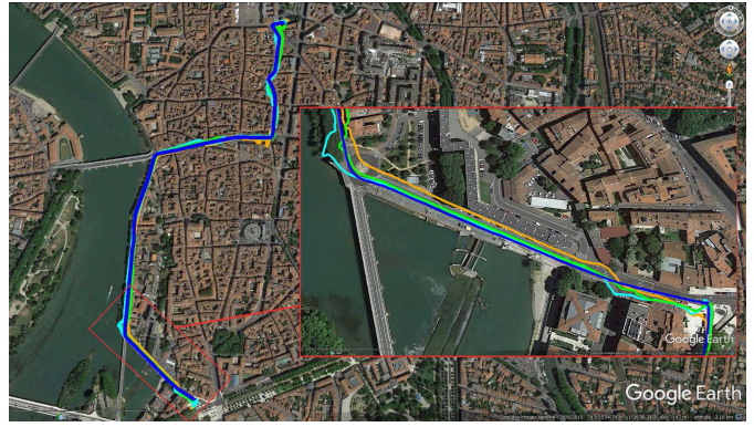
Fig. 20. Trajectory of the urban scenario plotted using Google Earth ® . The reference is in blue, the Ublox and REKF solutions are in green and orange, whereas the proposed method is in cyan.
