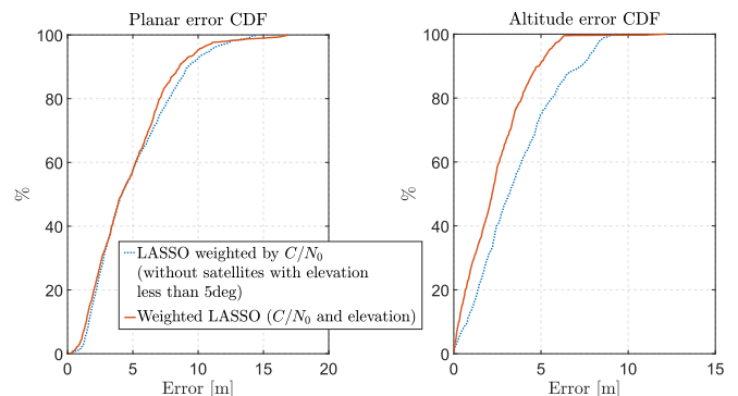
Fig. 11. Cumulative distribution functions of planar and altitude errors after weighting (continuous red) or discarding (blue dotted) low-elevation satellites.
