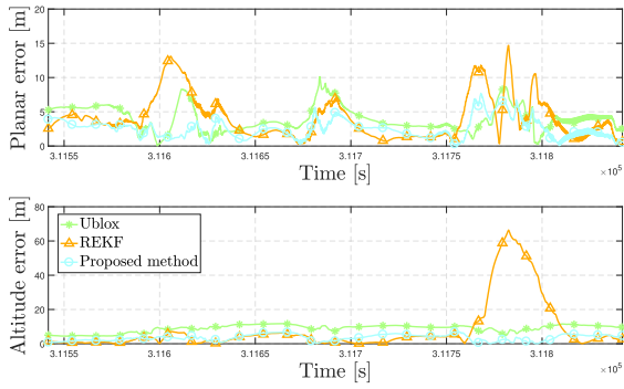
Fig. 18. Position errors versus time for the Ublox solution, the REKF and the proposed method for the open sky scenario.
