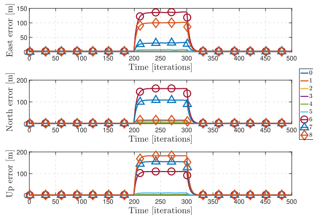
Fig. 10. Influence of the number of satellites affected by MP.
