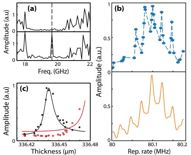
FIG. 2. (a) Zoom in of the acoustic spectrum around the fundamental cavity mode. The upper curve corresponds to an anti-resonant excitation with f_{\text{rep}} = 79.990 MHz and f^+/f_{\text{rep}} \approx 245 + 1/2 . The lower curve corresponds to a resonant excitation with f_{\text{rep}} = 80.130 MHz and f^+/f_{\text{rep}} \approx 245 . (b) Acoustic resonance amplitude as a function of the laser repetition rate. Measurement in upper curve and fit in lower curve. (c) Acoustic resonance amplitude as a function of the substrate thickness (proportional to the travel time). The experimental data (dots) and fit (line) are shown for the two signals resonant at f_m + f_{\text{mod}} in black and f_m - f_{\text{mod}} in red.
