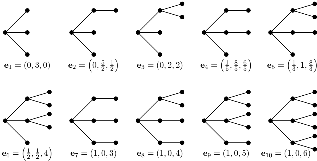
FIGURE 4. An enumeration of \mathbf{e}(T) for all trees T \in \mathcal{T}_2(3) .
