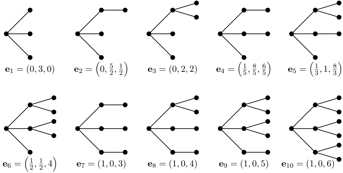
FIGURE 5. An enumeration of \mathbf{e}(T) for all trees T \in \mathcal{T}_2(3)
