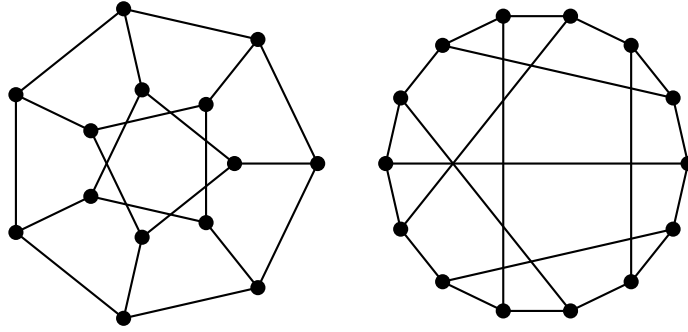
FIGURE 1. The two cubic triangle-free connected graphs with independence ratio \frac{5}{14} .
