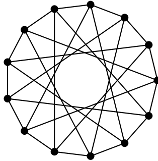
FIGURE 2. The only known 4-regular triangle-free connected graph of independence ratio \frac{4}{13} .
