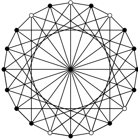
FIGURE 3. A 5-regular triangle-free (vertex-transitive) graph with independence ratio \frac{3}{10} . It is the Cayley graph over \mathbb{Z}_{20} with generating set \{\pm 1, \pm 6, \pm 10\} . There is no independent set of order 7, and the white vertices form an independent set of order 6.
