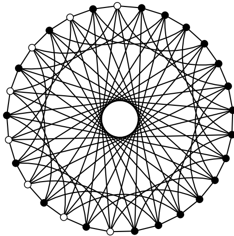
FIGURE 4. A 6-regular triangle-free (vertex-transitive) graph with independence ratio \frac{8}{29} . It is the Cayley graph over \mathbb{Z}_{29} with generating set \{\pm 1, \pm 5, \pm 13\} . There is no independent set of order 9, and the white vertices form an independent set of order 8.
