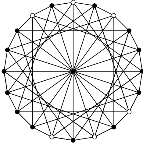
FIGURE 3. A 5-regular triangle-free (vertex-transitive) graph with independence ratio \frac{3}{10} . It has 20 vertices \{v_0, \dots, v_{19}\} with an edge between v_i and v_j if the (circular) distance between i and j in \mathbb{Z}_{20} is 1, 6 or 10. There is no independent set of order 7, and the white vertices form an independent set of order 6.
