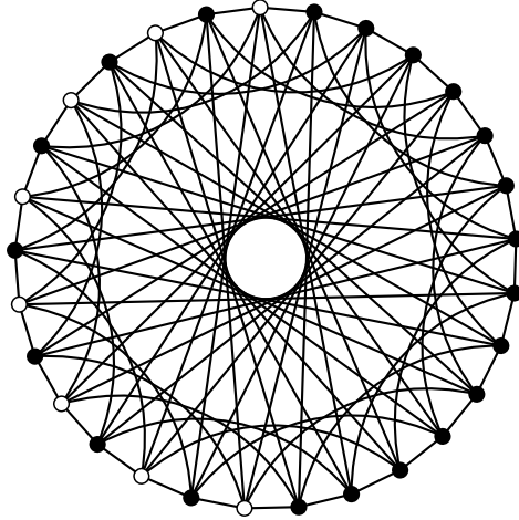
FIGURE 4. A 6-regular triangle-free (vertex-transitive) graph with independence ratio \frac{8}{29} . It has 29 vertices \{v_0, \dots, v_{28}\} with an edge between v_i and v_j if the (circular) distance between i and j in \mathbb{Z}_{29} is 1, 5 or 13. There is no independent set of order 9, and the white vertices form an independent set of order 8.
