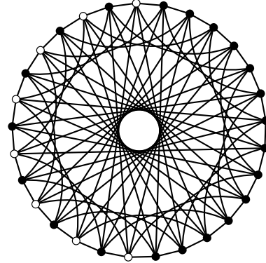
(B) A 6-regular triangle-free (vertex-transitive) graph with Hall ratio \frac{29}{8} . It is the Cayley graph over \mathbb{Z}_{29} with generating set \{\pm 1, \pm 5, \pm 13\} . There is no independent set of order 9, and the white vertices form a independent set of order 8.
