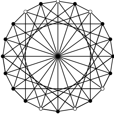
(A) A 5-regular triangle-free (vertex-transitive) graph with Hall ratio \frac{10}{3} . It is the Cayley graph over \mathbb{Z}_{20} with generating set \{\pm 1, \pm 6, \pm 10\} . There is no independent set of order 7, and the white vertices form a independent set of order 6.
