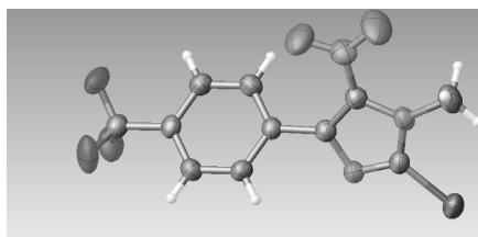
Figure 1. X-ray crystal structure of compound 3c .
