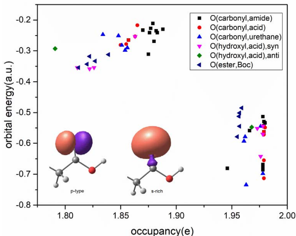
Figure 6. Scatter plot of occupancies and orbital energies of O lone pairs in the five compounds for O_{\text{carbonyl}} , O_{\text{hydroxyl}} , O_{\text{ester}} atoms. The shape of n_{\text{O}}^{(\pi)} (p-type) and n_{\text{O}}^{(\sigma)} s-rich lone pair lobes are shown at the bottom left corner in the graph. The n_{\text{O}}^{(\sigma)} lone pairs have lower occupancy and weaker energy in magnitude (less negative, clustered at left upper corner in the figure) compared to n_{\text{O}}^{(\pi)} lone pairs (right bottom corner).
