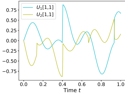
(a) Case 1: V_1(t) = \text{Span}(u_1(t)) and V_2(t) = \text{Span}(u_2(t)) . Discontinuities occur whenever \lambda_1(t) = \lambda_2(t) or \lambda_2(t) = \lambda_3(t) .
