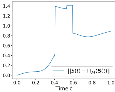
(b) Approximation error w.r.t. the exact re- (c) Errors w.r.t. the full \mathbf{S}(t) : dynamical error duction \Pi_{\mathcal{M}}(\mathbf{S}(t)) : i.e., \|\mathbf{S}(t) - \Pi_{\mathcal{M}}(\mathbf{S}(t))\| (blue) vs. best achievable error (orange).
