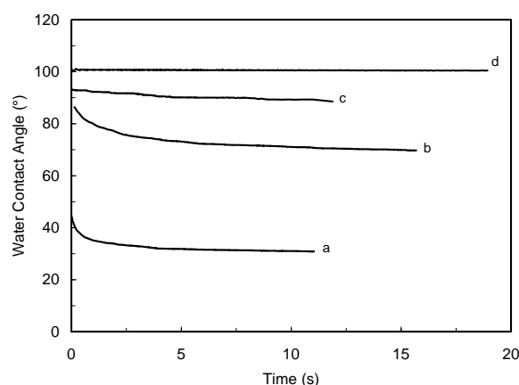
Figure 7: Water contact angle with time for unmodified ramie cellulose whiskers (a) and modified with hexanoyl chloride (b), lauroyl chloride (c) and stearyl chloride (d).
