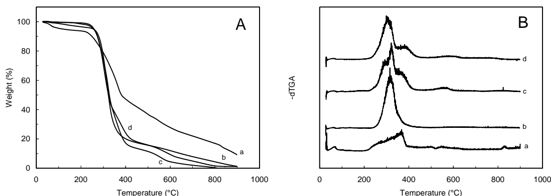
Figure 8: TGA curves (A) and dTGA (B) for unmodified ramie cellulose whiskers (a) and modified with hexanoyl chloride (b), lauroyl chloride (c) and stearoyl chloride
