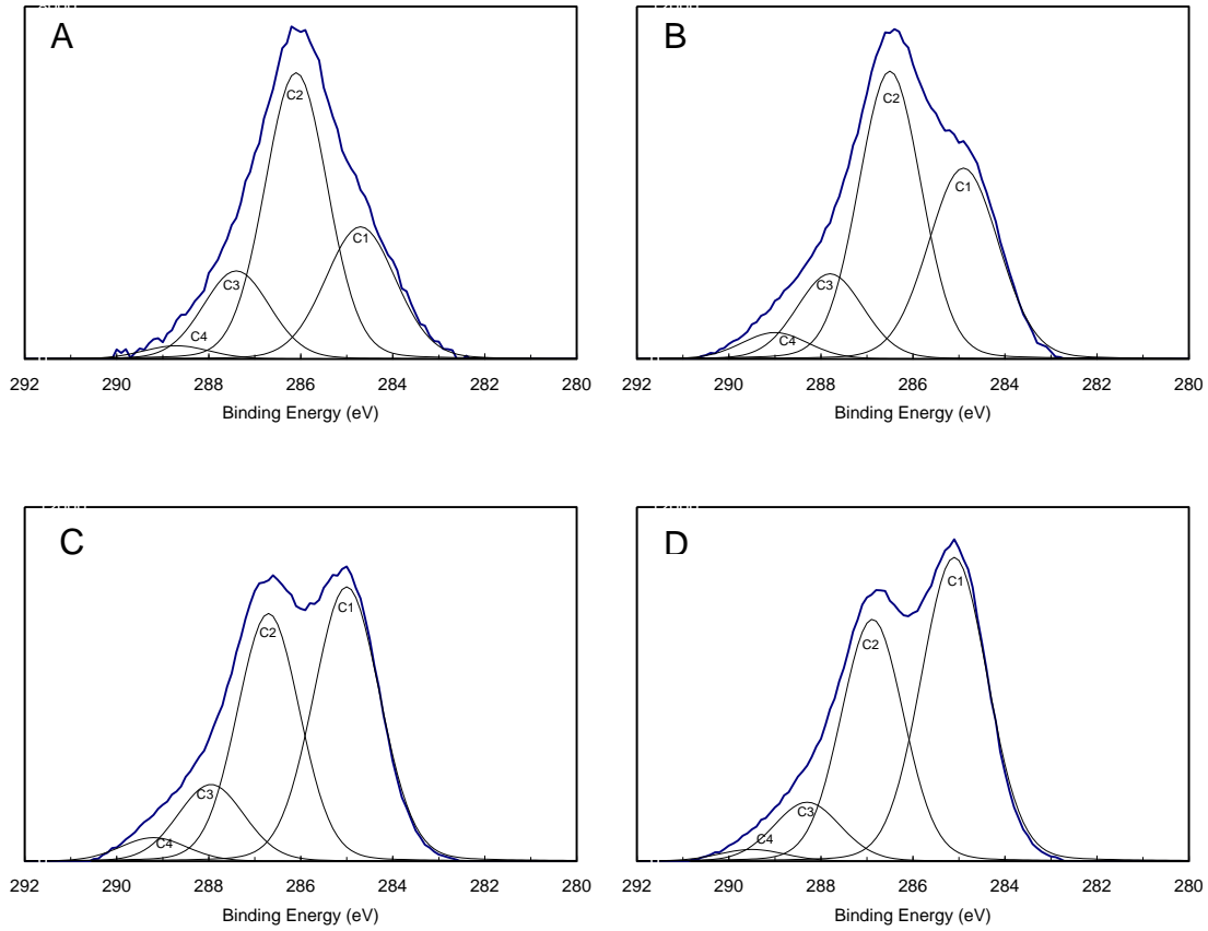
Figure 4: Decomposition of C1s signal into its constituent contributions for unmodified ramie cellulose whiskers (A) and modified with hexanoyl chloride (B), lauroyl chloride (C) and stearoyl chloride (D).
