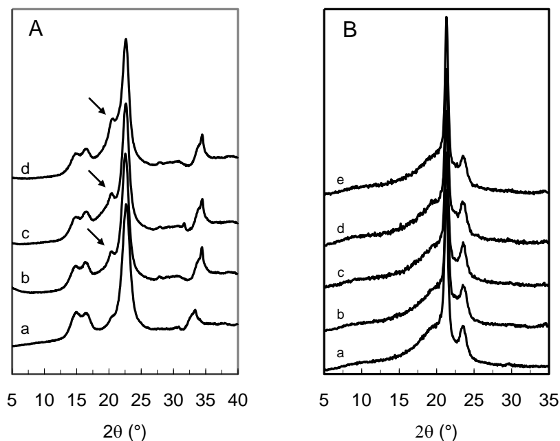
Figure 6: Wide-angle X-ray diffraction patterns for ramie cellulose whiskers (A): unmodified (a) and modified with hexanoyl chloride (b), lauroyl chloride (c) and stearoyl chloride (d), and nanocomposite films (B): neat LDPE matrix (a) and related nanocomposite films reinforced with 10 wt% ramie cellulose whiskers: unmodified (b) and modified with hexanoyl chloride (c), lauroyl chloride (d) and stearoyl chloride (e).
