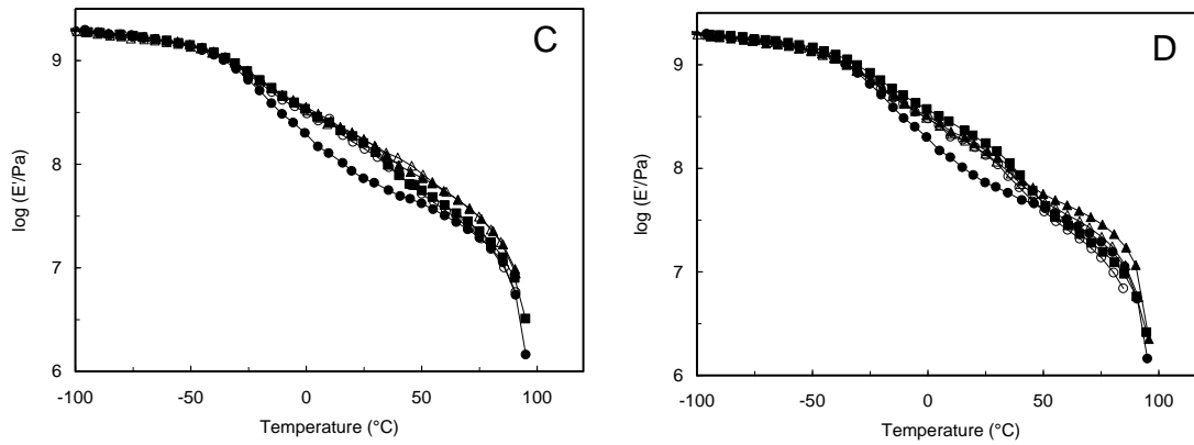
Figure 12: Evolution of the logarithm of the storage tensile modulus as a function of temperature for the neat LDPE matrix (●) and related nanocomposite films reinforced with 3 (A), 5 (B), 10 (C) and 15 wt% ramie cellulose whiskers: unmodified (○) and modified with hexanoyl chloride (▲), lauroyl chloride (△) and stearyl chloride (■).
