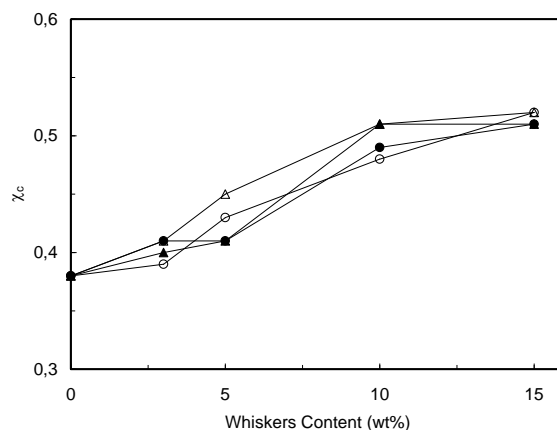
Figure 11: Evolution of the degree of crystallinity of the LDPE matrix as a function of the ramie cellulose whiskers content for nanocomposite films reinforced with unmodified (●) and modified with hexanoyl chloride (○), lauroyl chloride (▲) and stearyl chloride (Δ) whiskers.
