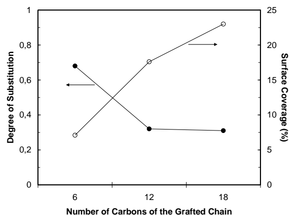
Figure 5: Evolution of the surface coverage area and degree of substitution (DS) as a function of the length of grafted chains. The lines serve to guide the eyes.
