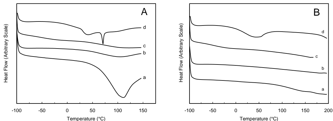
Figure 9: DSC traces for unmodified ramie cellulose whiskers (a) and modified with hexanoyl chloride (b), lauroyl chloride (c) and stearoyl chloride (d). First temperature scan (A) and second temperature scan recorded after the first temperature scan and subsequent quenching (B). Traces have been shifted vertically.
