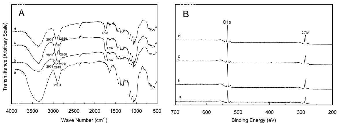
Figure 3: FTIR spectra (KBr pellets) (A) and general XPS spectra (B) of unmodified ramie cellulose whiskers (a) and surface modified with hexanoyl chloride (b), lauroyl chloride (c) and stearoyl chloride (d), after soxhlet extraction with acetone.
