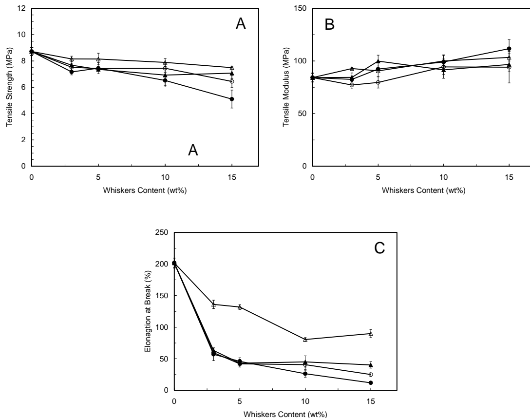
Figure 14: Evolution of the tensile strength (A), tensile modulus (B) and elongation at break (C) as a function of the ramie cellulose whiskers content for nanocomposite films reinforced with unmodified (●) and modified with hexanoyl chloride (○), lauroyl chloride (▲) and stearoyl chloride (△) whiskers. The lines serve to guide the eyes.
