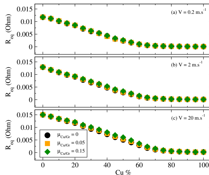
Figure 2. Evolution of the global electrical resistance for different Cu/Gr frictions (0, 0.05 and 0.15) and for different shear velocities: (a) 0.2 m/s; (b) 2 m/s; and (c) 20 m/s.
