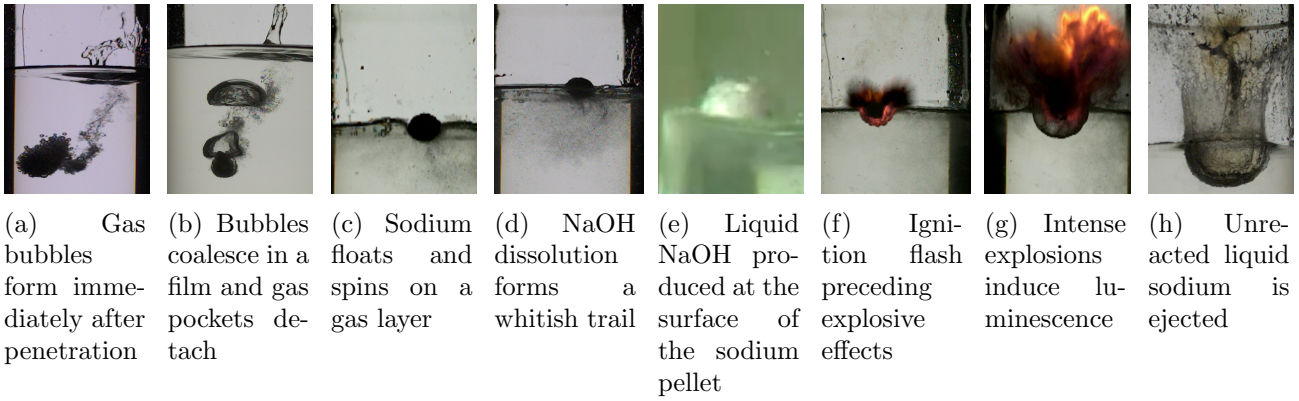
Figure 2: General observations made during reactions following the impact and penetration of 1 g sodium pellets in liquid water. The phenomenology depends on water temperature as discussed in Section 2.2.
