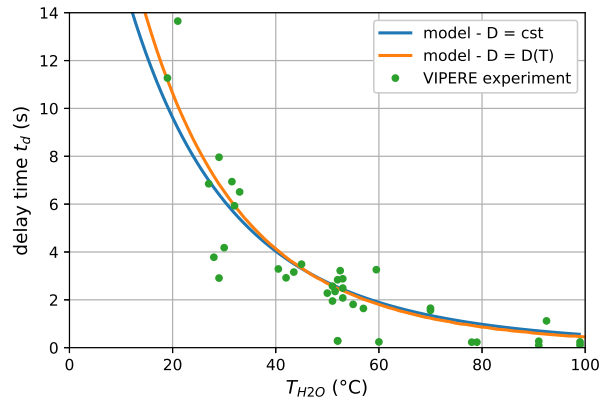
Figure 10: The trend obtained for the delay time is consistent with data from VIPERE experiments. If the parameter D is properly adjusted (by the least square method for example), quantitative agreement is also obtained.
