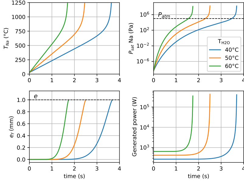
Figure 8: Results obtained by numerical resolution of eq. 10 for different water temperatures with D = 9.1 \text{ cm}^2 \text{ s}^{-1} , which display the same trends as experimental observations.
