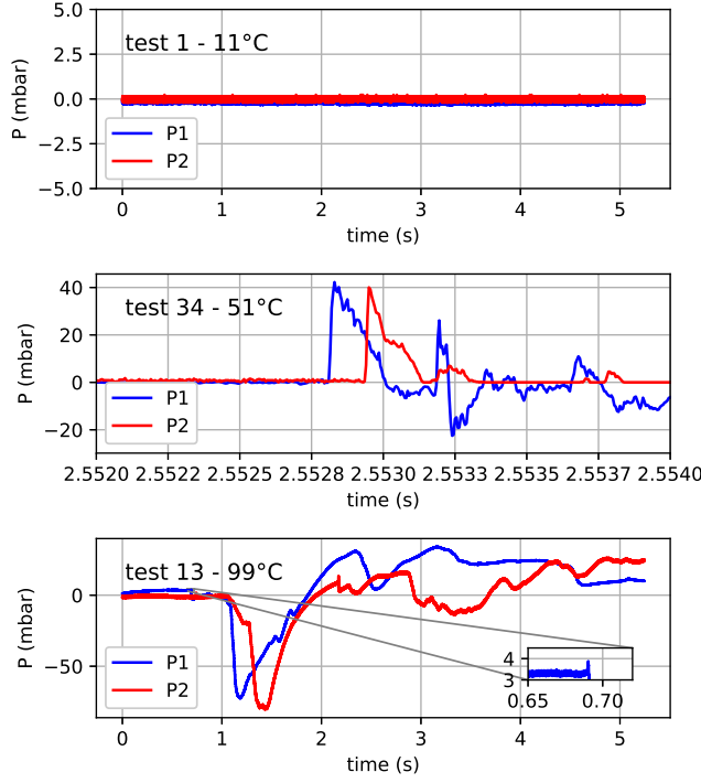
Figure 5: Three different types of typical pressure signals recorded during VIPERE experiments. The two sensors P1 and P2 are distant of 5 cm. Blast waves are recorded for intermediate water temperatures ( 27^\circ\text{C} < T_{\text{H}_2\text{O}} \leq 78^\circ\text{C} ). For lower temperatures, no pressure variation is recorded. For higher temperatures, weak explosions occur underwater and signals are damped. Only a small peak is detected followed by a depression due to the expansion of hot gases and to bubble collapse.
