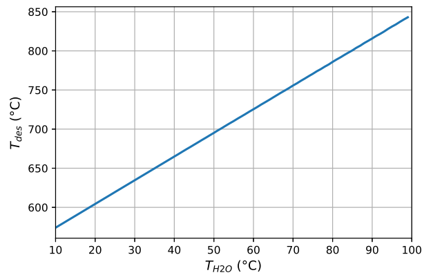
Figure 11: Destabilization temperature T_{des} grows linearly with water temperature and is close to sodium boiling temperature.
