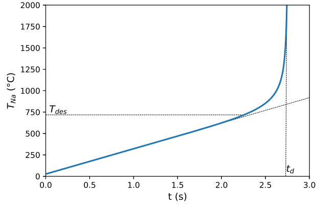
Figure 9: Definition of the destabilization temperature T_{des} and the delay time t_d .
