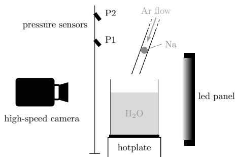
Figure 1: Schematic representation of VIPERE experimental setup. A 1 g spherical solid sodium pellet is put in contact with liquid water. The reaction is filmed using a high-speed camera.
