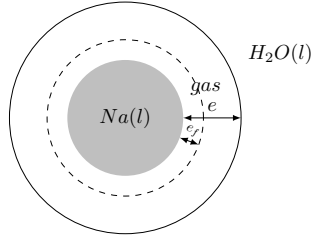
Figure 7: Configuration studied for the construction of the model. Sodium sample diameter is about 1 cm and film thickness e is about 1 mm.
