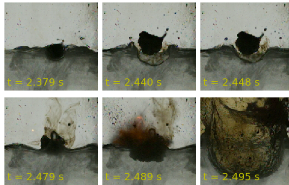
Figure 4: Apparition of a dark steam emanating from sodium in the instants preceding ignition (test 11, T_{H_2O} = 53^\circ\text{C} ).
