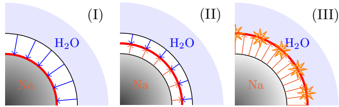
Figure 6: From left to right, the three step of the phenomenology postulated for SWR : (I) surface reaction, (II) gas-phase reaction, (III) runaway. The red surface symbolizes the reaction zone. The distinction between surface and gas-phase reactions during SWR was also made by Takata et al. [13].
