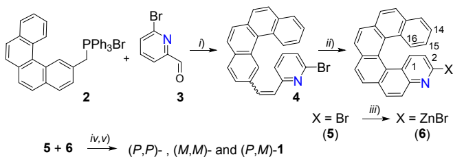
Scheme 2. Synthesis of 1 as a mixture of (P,P) , (M,M) , and (P,M) stereoisomers. i) n -BuLi, THF, rt, Ar, 5 hrs, 90%; ii) h\nu , I_2 (2 equiv.), propylene oxide (49 equivs), toluene, rt, Ar, 15 hrs, 45%; iii) n -BuLi, ZnCl_2 , THF, rt, Ar, 5 hrs, 90%; iv) Pd(PPh_3)_4 , THF, reflux, Ar, 15 hrs; v) TPEN, CH_2Cl_2 , 57% (two steps).
