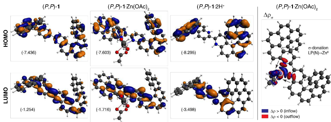
Figure 3. Left: Isosurfaces ( \pm 0.03 au) of frontier MOs of the bis-helical bipyridine ligand 1 , of its corresponding Zn complex 1 \cdot Zn(OAc)_2 , and of its doubly protonated species 1 \cdot 2H^+ . Right: Isosurface ( \pm 0.0015 au) of dominant ETS-NOCV deformation density channel depicting formation of the 1 \cdot Zn(OAc)_2 bonding. Only the most populated (lowest-energy) conformers' results have been shown; see SI for a full set of data.
