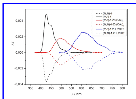
Figure 6. CPL spectra of (P,P)\text{-}1 (solid black), its Zn complex (P,P)\text{-}1 \cdot \text{Zn}(\text{OAc})_2 (solid red), and its fully protonated species (P,P)\text{-}1 \cdot 2\text{H}^+ , 2\text{OTf}^- along with the corresponding spectra of their mirror-images (dash lines) measured in \text{CH}_2\text{Cl}_2 at rt ( C \approx 1 \times 10^{-5} \text{M} ). Excitation wavelengths: \lambda_{\text{ex}} at 350 nm for 1 and 1 \cdot \text{Zn}(\text{OAc})_2 ; 460 nm for 1 \cdot 2\text{H}^+ , 2\text{OTf}^- . Maximum intensities have been normalized to 2.
