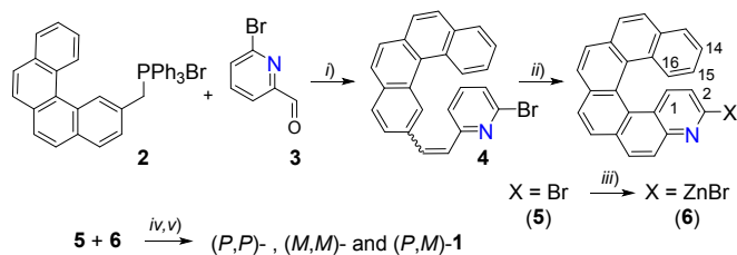
Scheme 2. Synthesis of 1 as a mixture of ( P,P ), ( M,M ), and ( P,M ) stereoisomers. i) n -BuLi, THF, rt, Ar, 5 hrs, 90%; ii) hv, I 2 (2 equiv.), propylene oxide (49 equivs), toluene, rt, Ar, 15 hrs, 45%; iii) n -BuLi, ZnCl 2 , THF, rt, Ar, 5 hrs, 90%; iv) Pd(PPh 3 ) 4 , THF, reflux, Ar, 15 hrs; v) TPEN, CH 2 Cl 2 , 57% (two steps).
