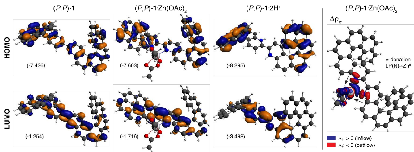
Figure 3. Left: Isosurfaces (±0.03 au) of frontier MOs of the bis-helical bipyridine ligand 1 , of its corresponding Zn complex 1 ·Zn(OAc) 2 , and of its doubly protonated species 1 ·2H + . Right: Isosurface (±0.0015 au) of dominant ETS-NOCV deformation density channel depicting formation of the 1 -Zn(OAc) 2 bonding. Only the most populated (lowest-energy) conformers' results have been shown; see SI for a full set of data.
