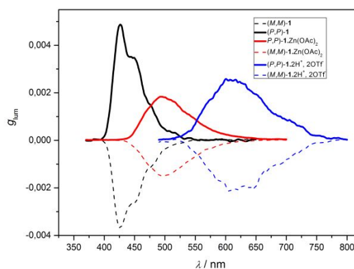
Figure 6. CPL spectra of (P,P) - 1 (solid black), its Zn complex (P,P) - 1 \cdot \text{Zn}(\text{OAc})_2 (solid red), and its fully protonated species (P,P) - 1 \cdot 2\text{H}^+ \cdot 2\text{OTf} along with the corresponding spectra of their mirror-images (dash lines) measured in \text{CH}_2\text{Cl}_2 at rt ( C \sim 1 \times 10^{-5} \text{M} ). Excitation wavelengths: \lambda_{\text{exc}} at 350 nm for 1 and 1 \cdot \text{Zn}(\text{OAc})_2 , and 460 nm for 1 \cdot 2\text{H}^+ \cdot 2\text{OTf} .
