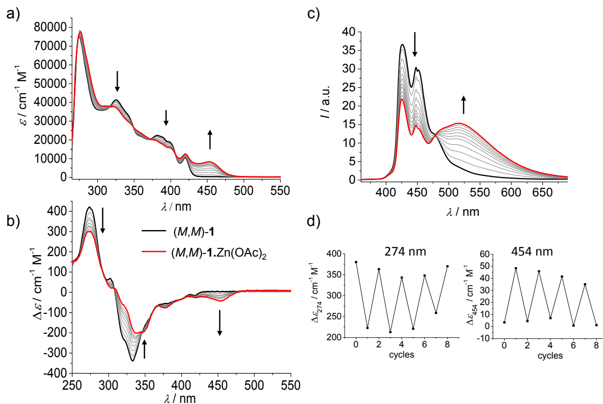
Figure 4. Evolution of UV/Vis spectrum of ( P*,P* )- 1 17 (panel a) and ECD spectrum of ( M,M )- 1 (panel b) upon addition of Zn(OAc) 2 ·2H 2 O aliquots (0.2 equiv. until saturation at 1.0-1.2 equivs; C 3 × 10 -5 M, CH 2 Cl 2 , rt). Panel c: Evolution of fluorescence of ( P*,P* )- 1 17 (λ ex = 350 nm, C 2.2 × 10 -5 M, CH 2 Cl 2 , rt). Panel d: Reversible ECD 274nm and ECD 454nm switching process.
