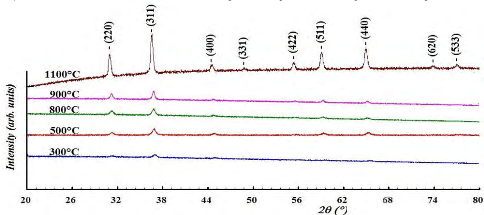
Figure 2: Powder X-ray diffraction pattern of \text{CoAl}_2\text{O}_4 prepared at \text{pH}=7 and calcined for 5h at different temperatures.
