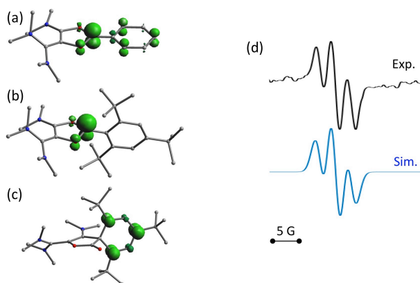
Figure 4: Representation of computed Mulliken spin densities for, (a) 6a , (b) 6d and (c) 11d ; (d) Experimental X-band isotropic EPR spectrum at room temperature in acetonitrile after reduction of 6d (top, in black), the simulated spectrum (bottom, in blue) was obtained with a Lorentzian line-broadening parameter of 0.25 and an hyperfine constant a(^1\text{H}) of 8.0 MHz (2 nuclei).
