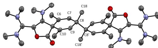
Figure 3: Representation of the X-ray structure of 9b with 50% probability ellipsoids. Counter-anions, hydrogen atoms and solvent are omitted for clarity.
