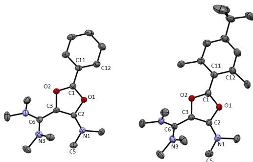
Figure 1: Representation of the X-ray structure of 6a and 6c with 50% probability ellipsoids. Counter-anions, hydrogen atoms and solvent are omitted for clarity. See Table 1 for key structural parameters.
