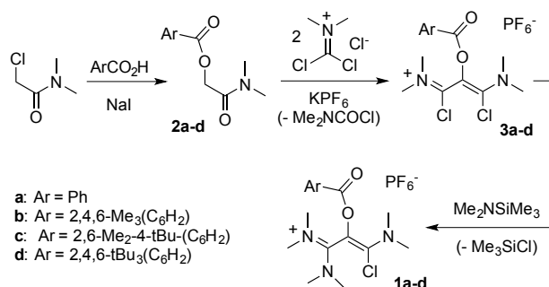
Scheme 2: Synthesis of 1-(chloro)vinamidinium salts 1a-d .
