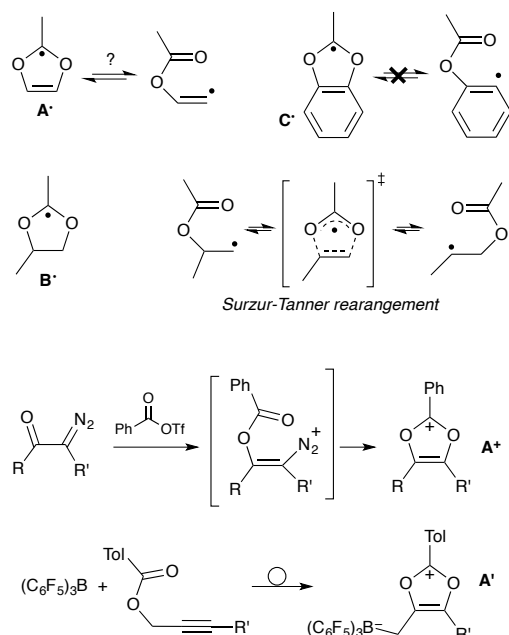
Scheme 1. Dioxolyl, dioxolanyl and benzodioxolyl radicals A • - C • ; their relation with "Surzur-Tanner"-type rearrangements; synthesis of dioxoliums salts A + and A' .
