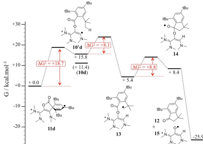
Figure 5: Computed mechanism for the formation of indanone 12 from 11d at the; u\omega\text{B97XD}/6\text{-}311\text{g(d,p)}/\text{PCM}(\text{acetonitrile}) level of theory relative Gibbs energies of intermediates and Gibbs energies of activation.
