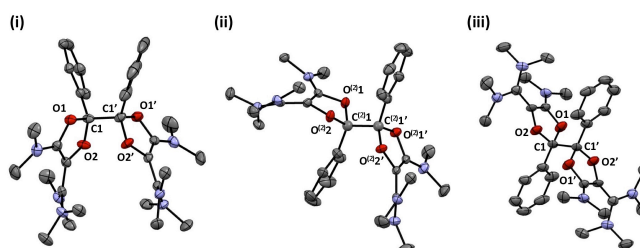
Figure 2: Representation of the X-ray structure of d,l - 8a (i: gauche conformer; ii: anti conformer) and meso - 8a (iii) with 50% probability ellipsoids. Counter-anions, hydrogen atoms and solvent are omitted for clarity.
