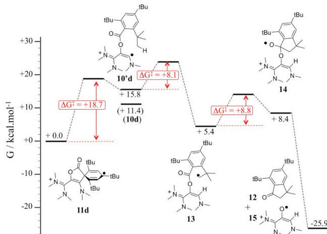
Figure 5: Computed mechanism for the formation of indanone 12 from 11d at the; u\omega\text{B97XD/6-311g(d,p)/PCM(acetonitrile)} level of theory relative Gibbs energies of intermediates and Gibbs energies of activation.
