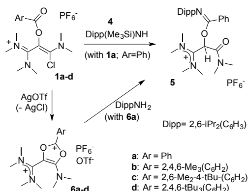
Scheme 3: Reaction of \mathbf{1a} with trimethylsilylanilines; synthesis of dioxolium salts \mathbf{6a-d} .
