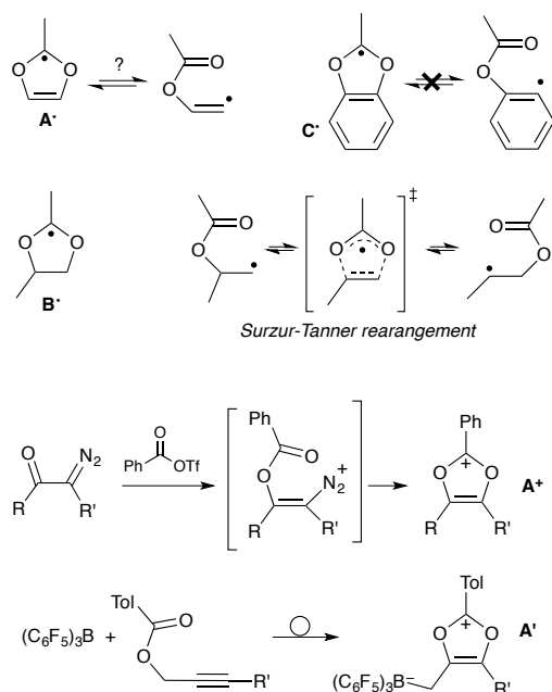
Scheme 1. Dioxoly, dioxolanyl and benzodioxoly radicals A • - C • ; their relation with "Surzur-Tanner"-type rearrangements; synthesis of dioxoliums salts A + and A' .
