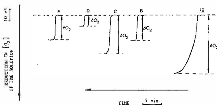
Fig. 4. Curves of absorption of oxygen in microemulsions B, C, D and E (reference C_4F_9-CH=CH-C_4F_9 ).
