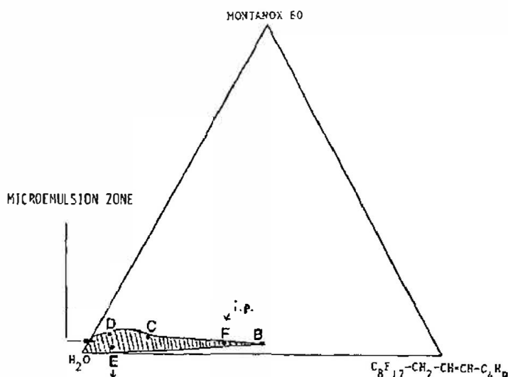
Fig. 3. Pseudoternary phase diagram of the system H_2O -Montanox 80- C_8F_{17}-CH_2-CH=CH-C_4H_9 .
