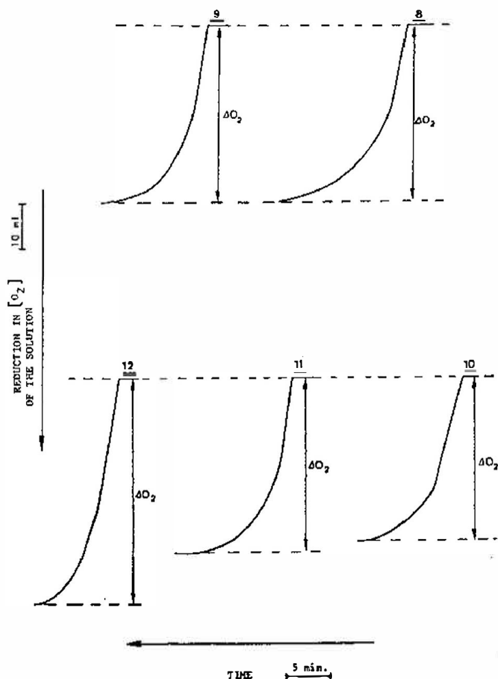
Fig. 1. Absorption of oxygen in 5 commercially available fluorinated oils. Calibration curves.
