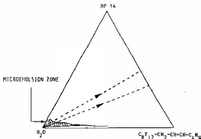
Fig. 2. Pseudoternary phase diagram of the system H 2 O-NP14-C 8 F 17 -CH 2 -CH=CH-C 4 H 9 (NP14 = C 9 H 19 -C 6 H 4 -(O-CH 2 -CH 2 ) 14 OH).
