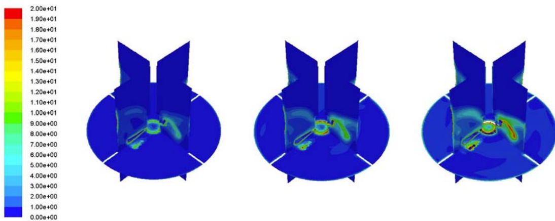
Fig. 4: Space distributions of the turbulent dissipation rate, \epsilon ( m^2/s^3 ), at 600 rpm (left), 700rpm (center), 800 rpm (right) according to water-phase CFD simulation.
