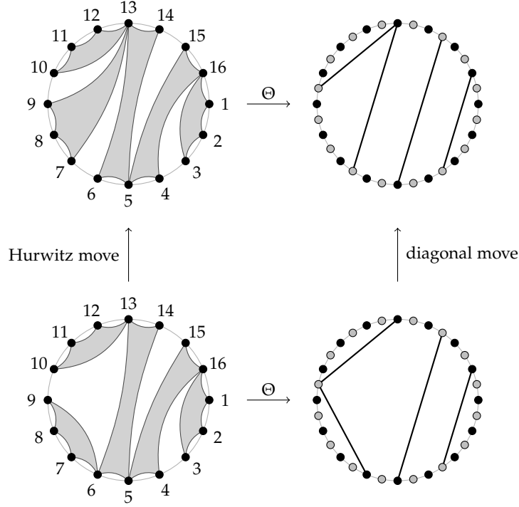
FIGURE 4. Illustration of the bijection \Theta from Theorem 6.4 for n = 5 and k = 3 .
