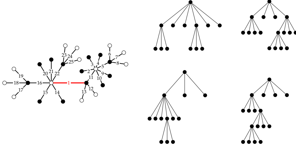
FIGURE 3. Illustration of the bijection from Theorem 1.2 for n = 8 , k = 3 , and w = (1\ 14\ 15\ 16\ 20\ 21\ 22)(2\ 3\ 4\ 5\ 9\ 10\ 11) \in \text{NC}_{25,3} . On the left is the plane, edge-rooted bicolored tree corresponding to w \cdot \text{Krew}(w) , in the middle the pair of 3-divisible trees with a total of 26 vertices, and on the right the pair of 4-ary trees with a total of 8 non-leaf vertices.
