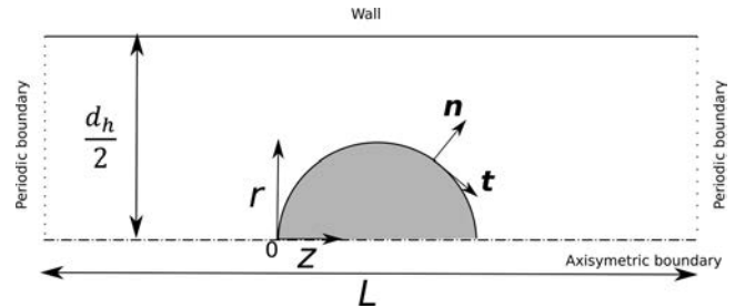
Figure 1. Axisymmetric bubble of density \rho_d and viscosity \mu_d immersed in a viscous liquid of density \rho_c and viscosity \mu_c inside a cylindrical microchannel of length L and diameter d_h . The unit vector normal to the gas–liquid interface, n , and the unit vector tangent to the gas–liquid interface, t , are sketched in this figure.
