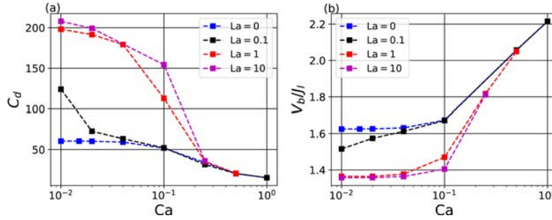
Figure 13. (a) Drag coefficient as a function of Ca for d/d_h = 0.75 and different values of La . (b) V_b/J_1 as a function of Ca for d/d_h = 0.75 and different values of La .
