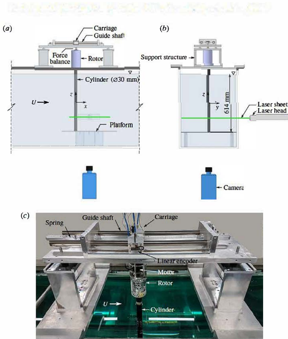
FIGURE 2. (Colour online) Schematics of the experimental set-up are shown in (a) side view and (b) back view. A photograph of the rig placed on top of the water channel is shown in (c).
