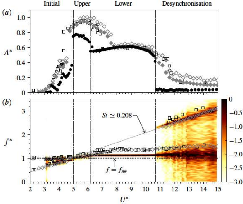
FIGURE 3. (Colour online) Structural vibration of non-rotating cylinders undergoing VIV. (a) The normalised amplitude response as a function of the reduced velocity. The solid circles (●) represent the mean of the highest 10% of the amplitudes ( A_{10}^* ) at each U^* in the present study, with m^* = 5.73 and \zeta = 2.44 \times 10^{-3} ; the open diamonds (◇) and solid diamonds (◆) represent the A_{max}^* and A_{10}^* values, respectively, in Zhao et al. (2014b), with m^* = 2.40 and \zeta = 2.43 \times 10^{-3} ; the open squares (□) represent the A_{max}^* values in Khalak & Williamson (1997), with m^* = 2.4 and \zeta = 4.5 \times 10^{-3} . (b) The corresponding frequency responses of the previous studies overlapped on the logarithmic-scale power spectral density contour of the present study. It should be noted that the power spectral density is normalised by the maximum value at each U^* .
