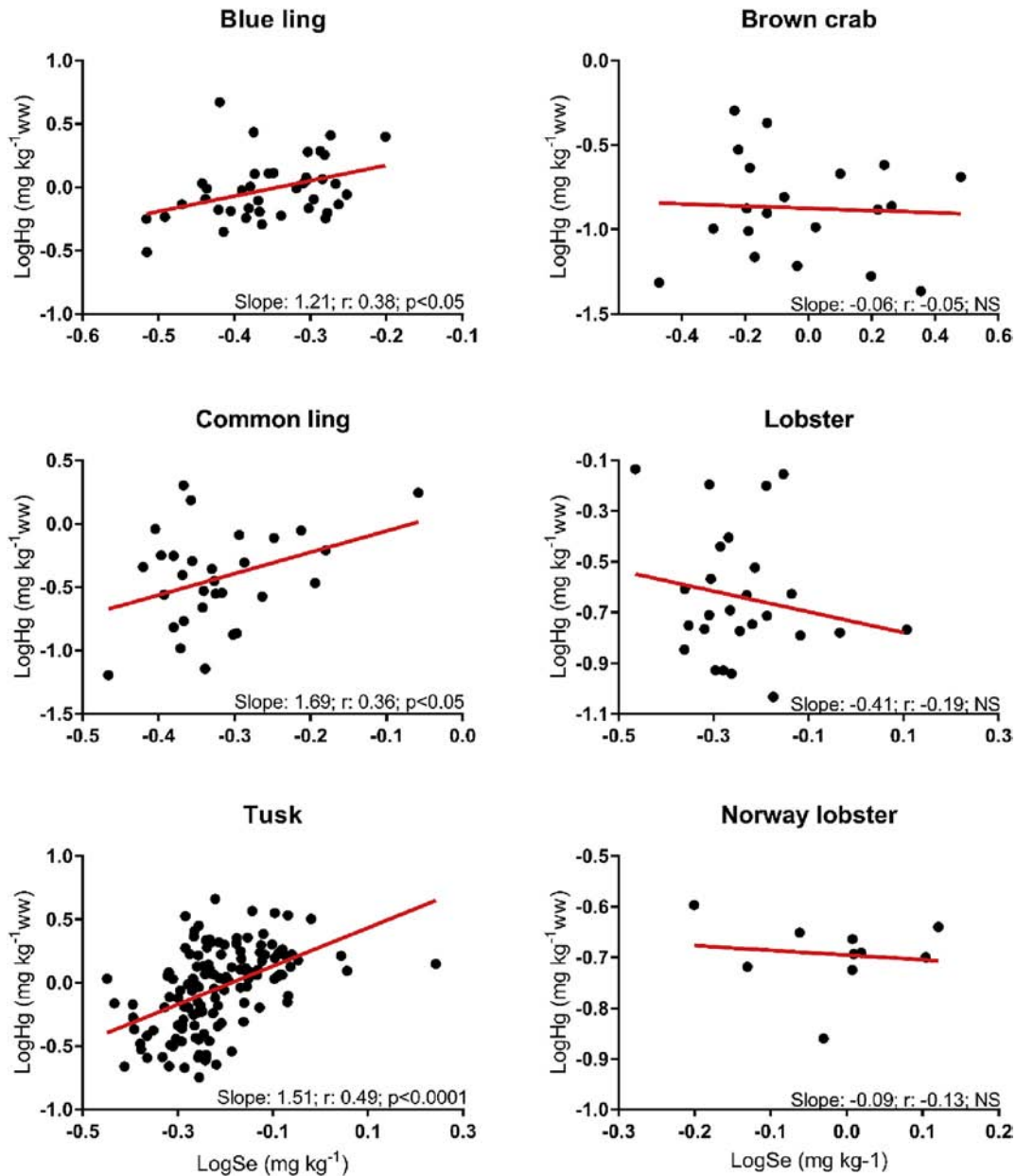
Fig. 3. Relationship between log Hg and log Se ( \text{mg kg}^{-1} ww) in fish and crustacean species from Hardangerfjord, 2011. Slope, r and P are presented. NS = not significant.
